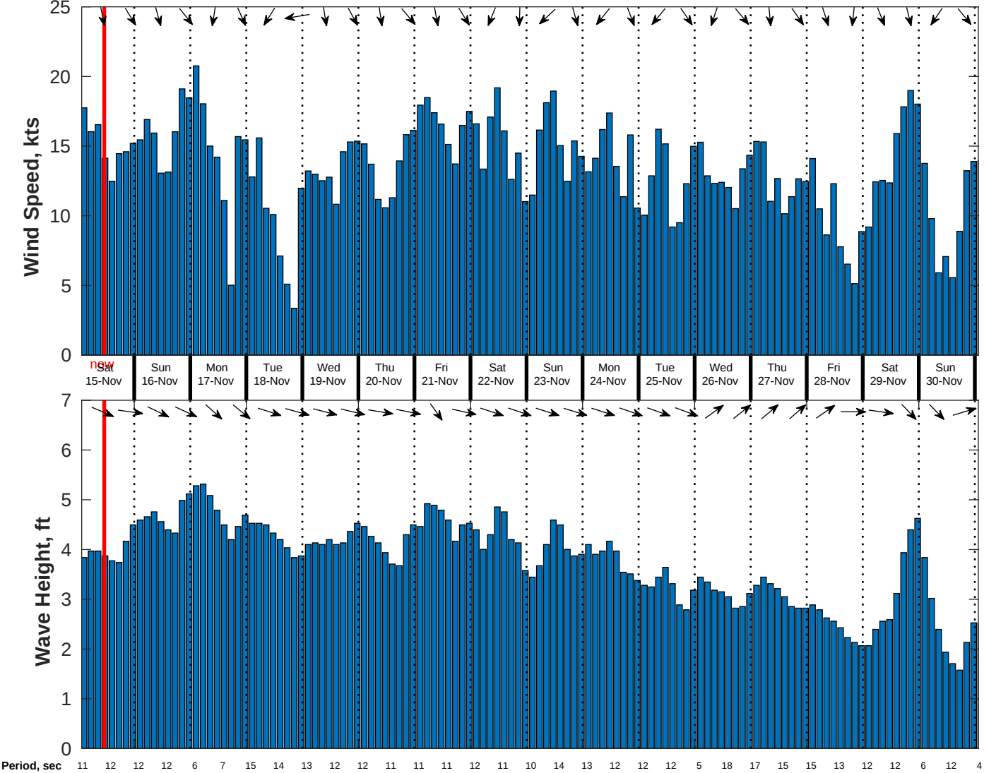
Wind & Wave Forecast for CSA (ONHYM) PPL EBS - Mauritania from 14-Nov-2025 01:00:00 to 30-Nov-2025 01:00:00
