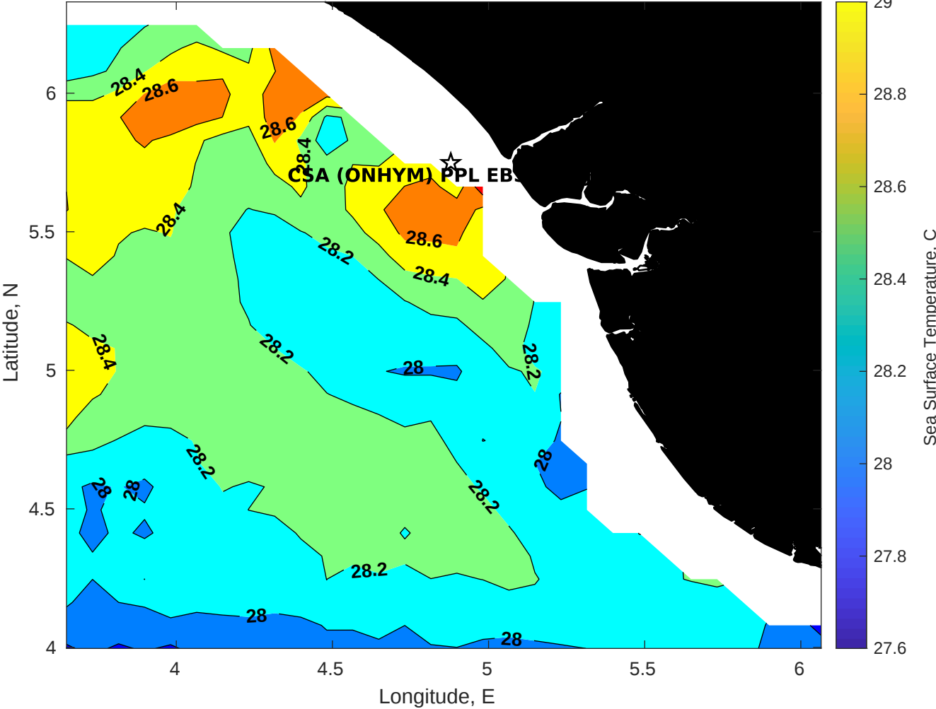
SST for CSA (ONHYM) PPL EBS - Nigeria at 14-Nov-2025 00:00:00
