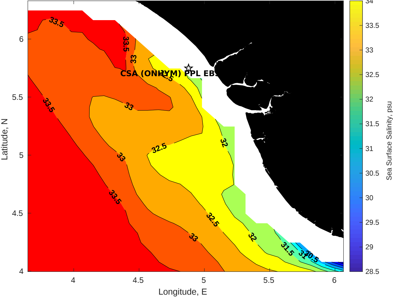
Surface Salinity for CSA (ONHYM) PPL EBS - Nigeria at 14-Nov-2025 00:00:00
