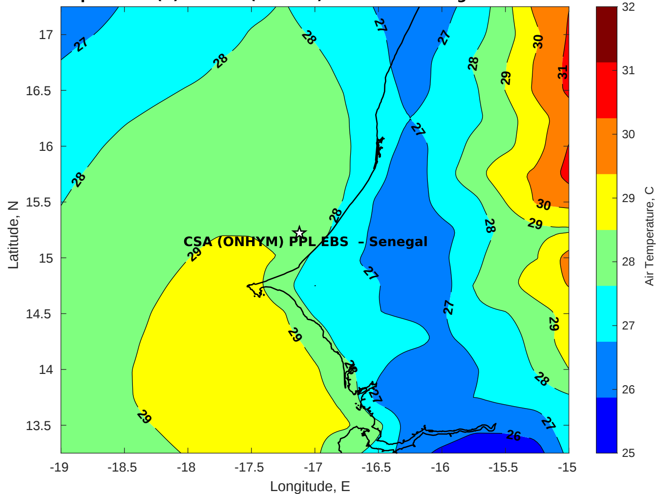
Air Temperature (C) for CSA (ONHYM) PPL EBS - Senegal at 15-Nov-2025
