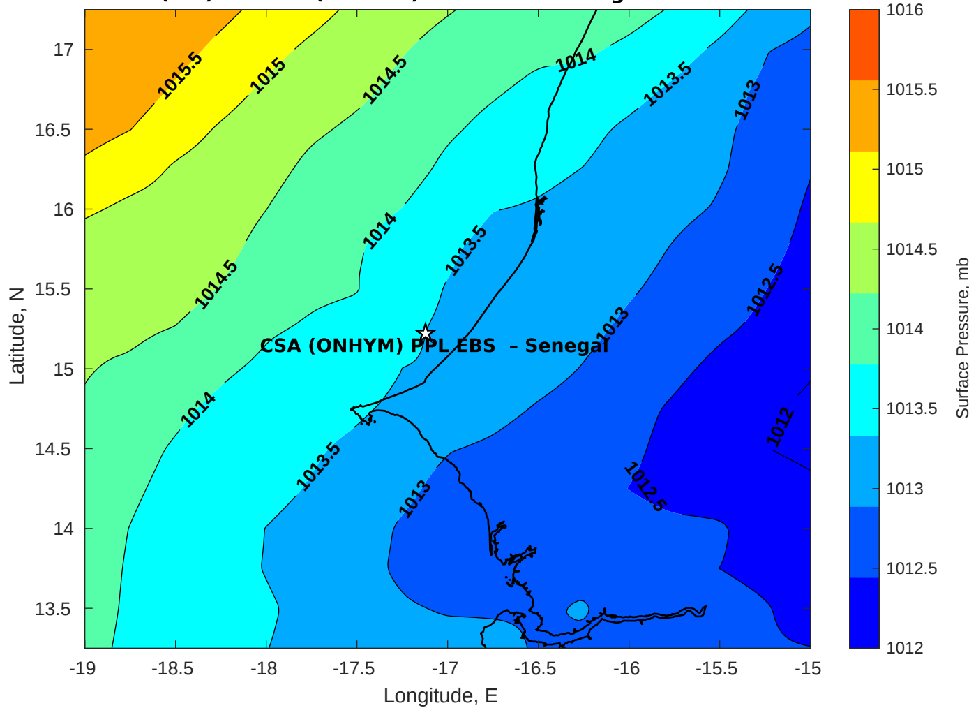
Surface Pressure (mb) for CSA (ONHYM) PPL EBS - Senegal at 15-Nov-2025 00:00:00
