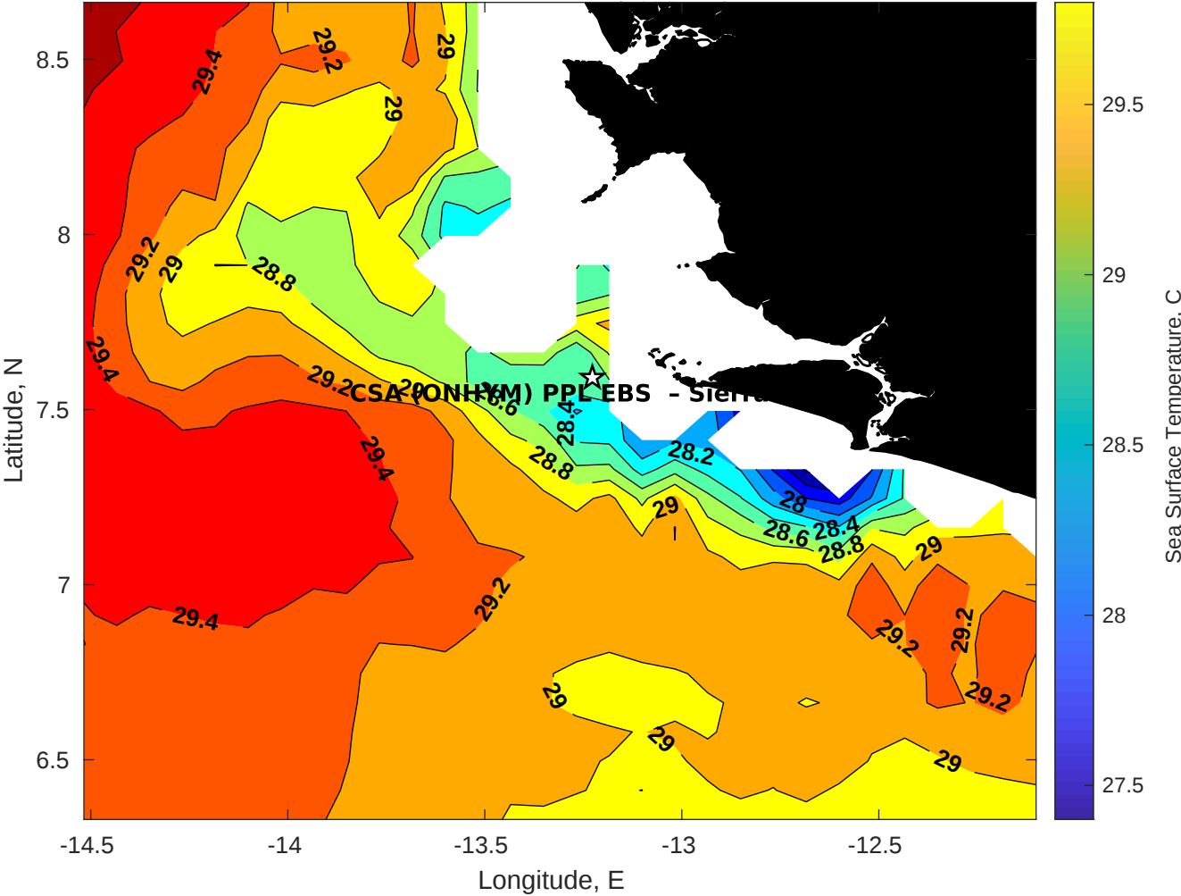
SST for CSA (ONHYM) PPL EBS - Sierra Leone at 14-Nov-2025 00:00:00
