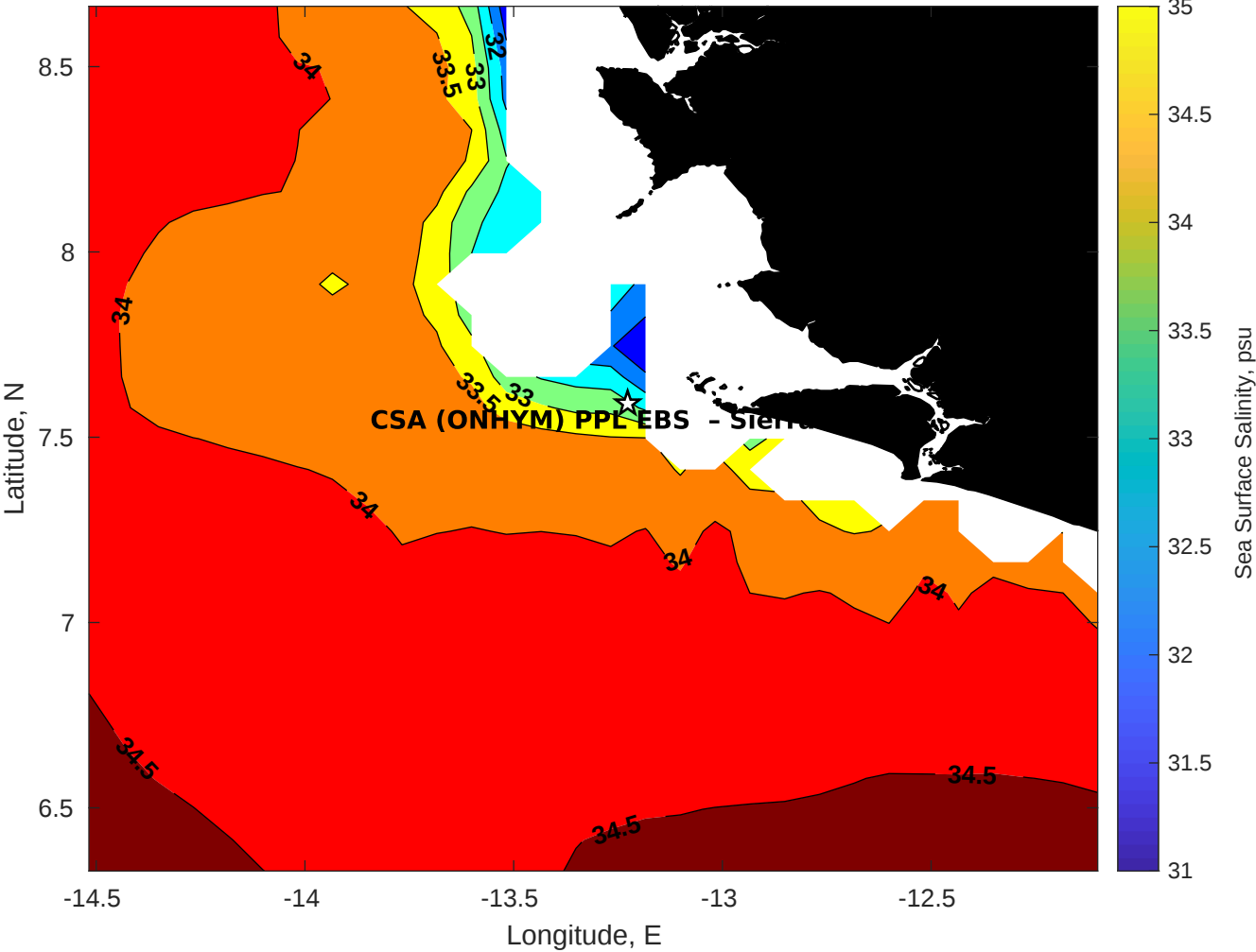
Surface Salinity for CSA (ONHYM) PPL EBS - Sierra Leone at 14-Nov-2025 00:00:00
