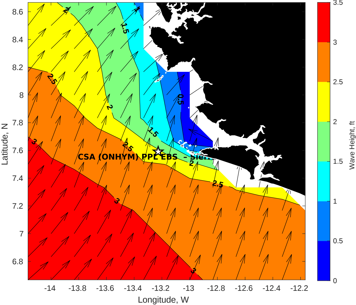
Wave Height (ft) for CSA (ONHYM) PPL EBS - Sierra Leone at 15-Nov-2025 09:00:00
