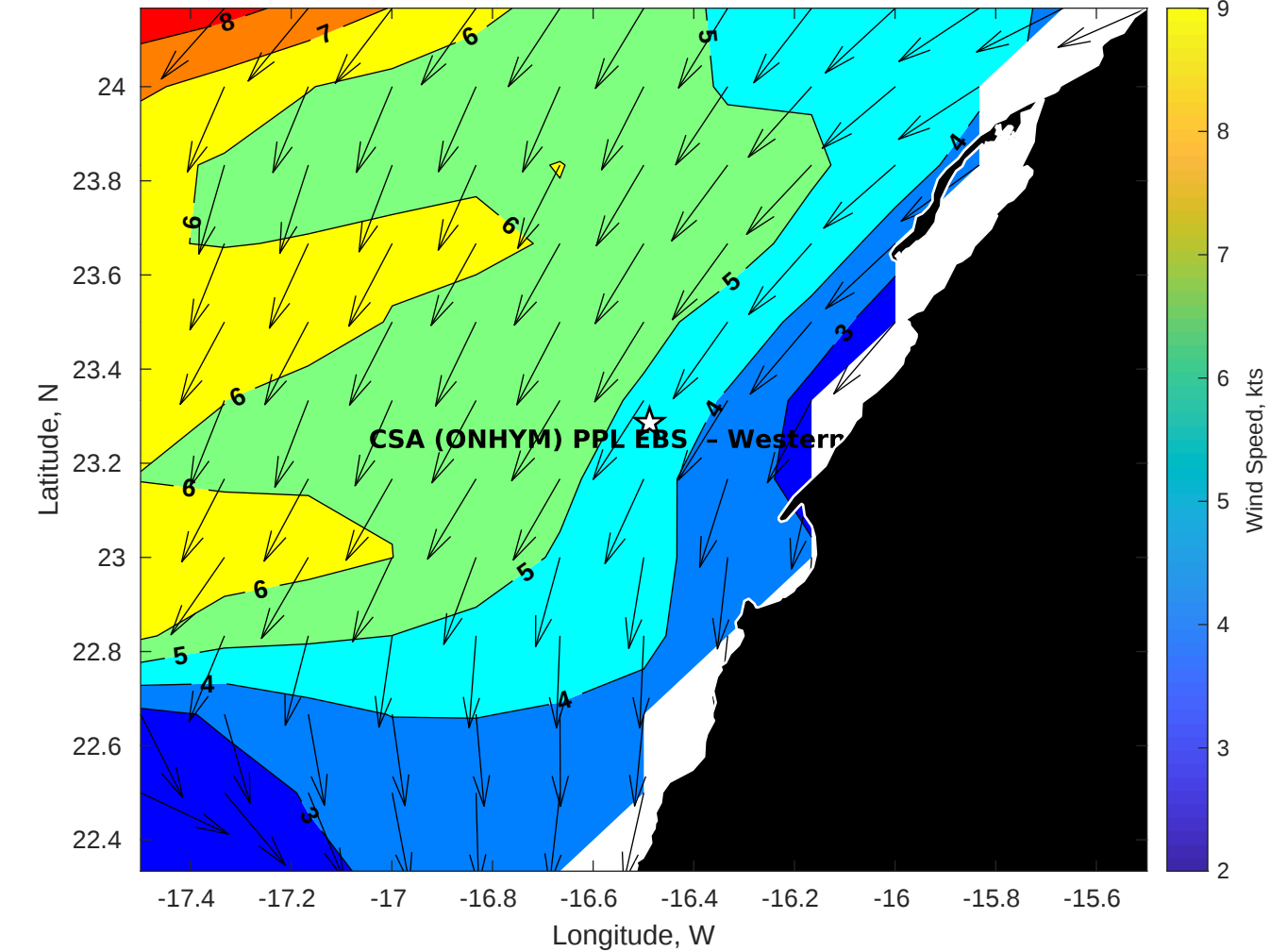
Winds (kts) for CSA (ONHYM) PPL EBS - Western Sahara at 14-Nov-2025 09:00:00
