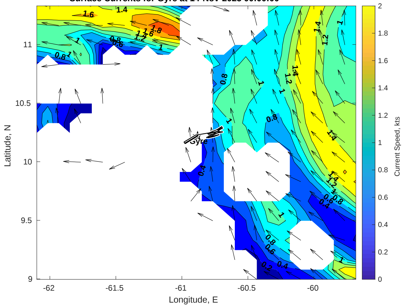
Surface Currents for Gyre at 14-Nov-2025 00:00:00
