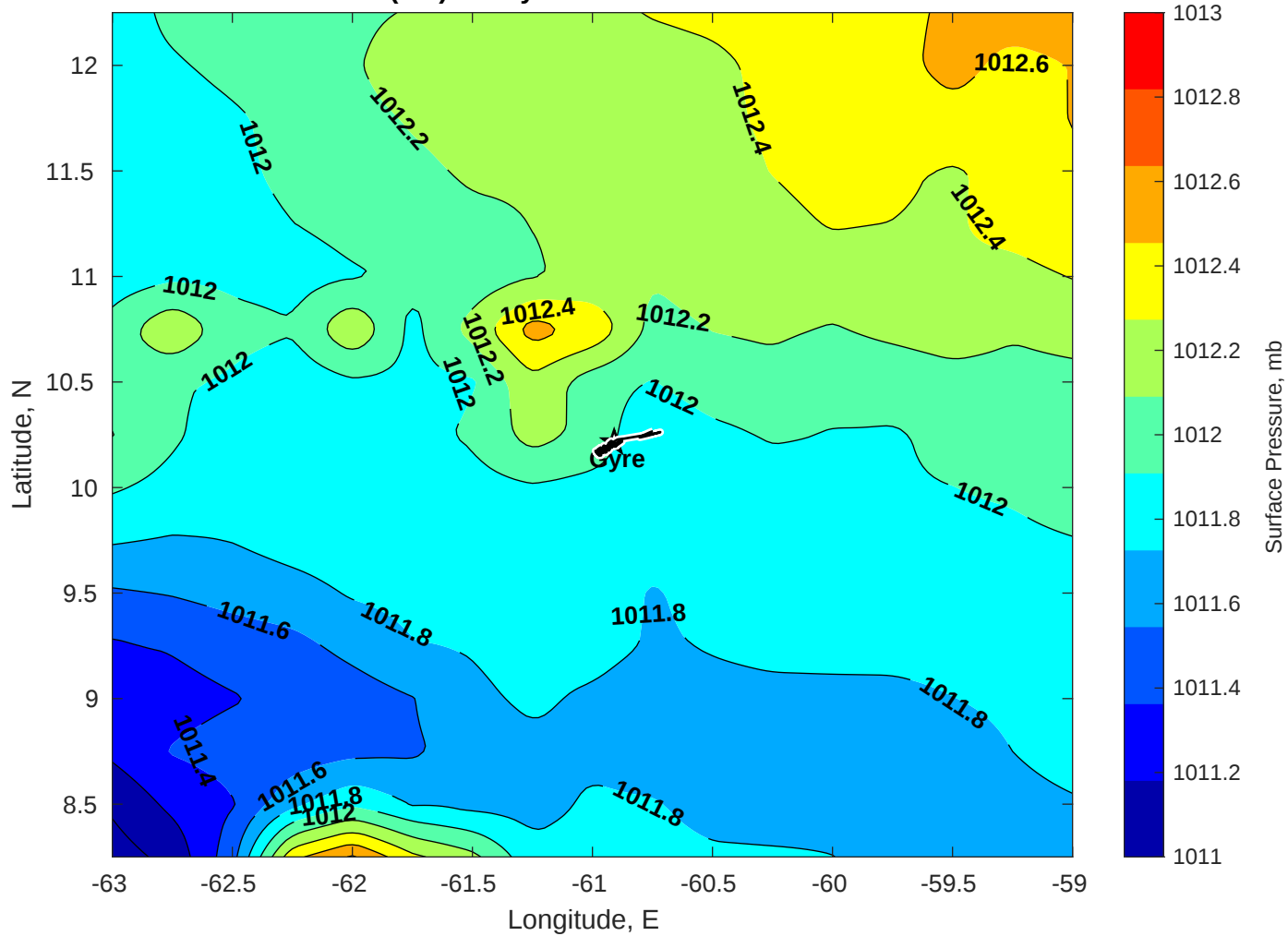
Surface Pressure (mb) for Gyre at 15-Nov-2025 00:00:00
