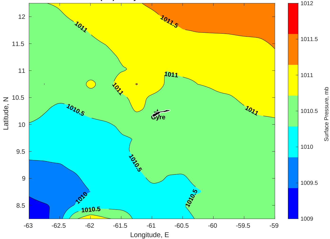
Surface Pressure (mb) for Gyre at 16-Nov-2025 00:00:00
