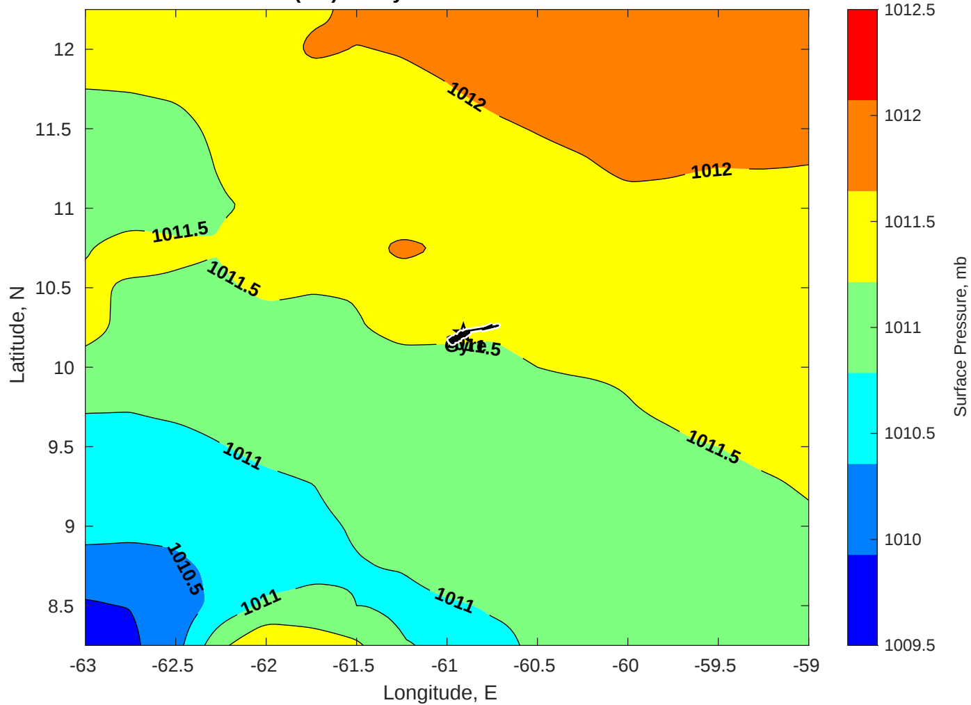
Surface Pressure (mb) for Gyre at 17-Nov-2025 00:00:00
