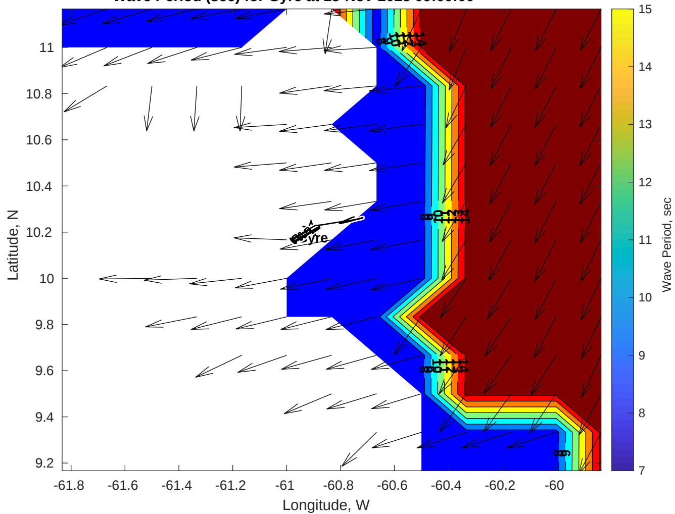
Wave Period (sec) for Gyre at 15-Nov-2025 09:00:00
