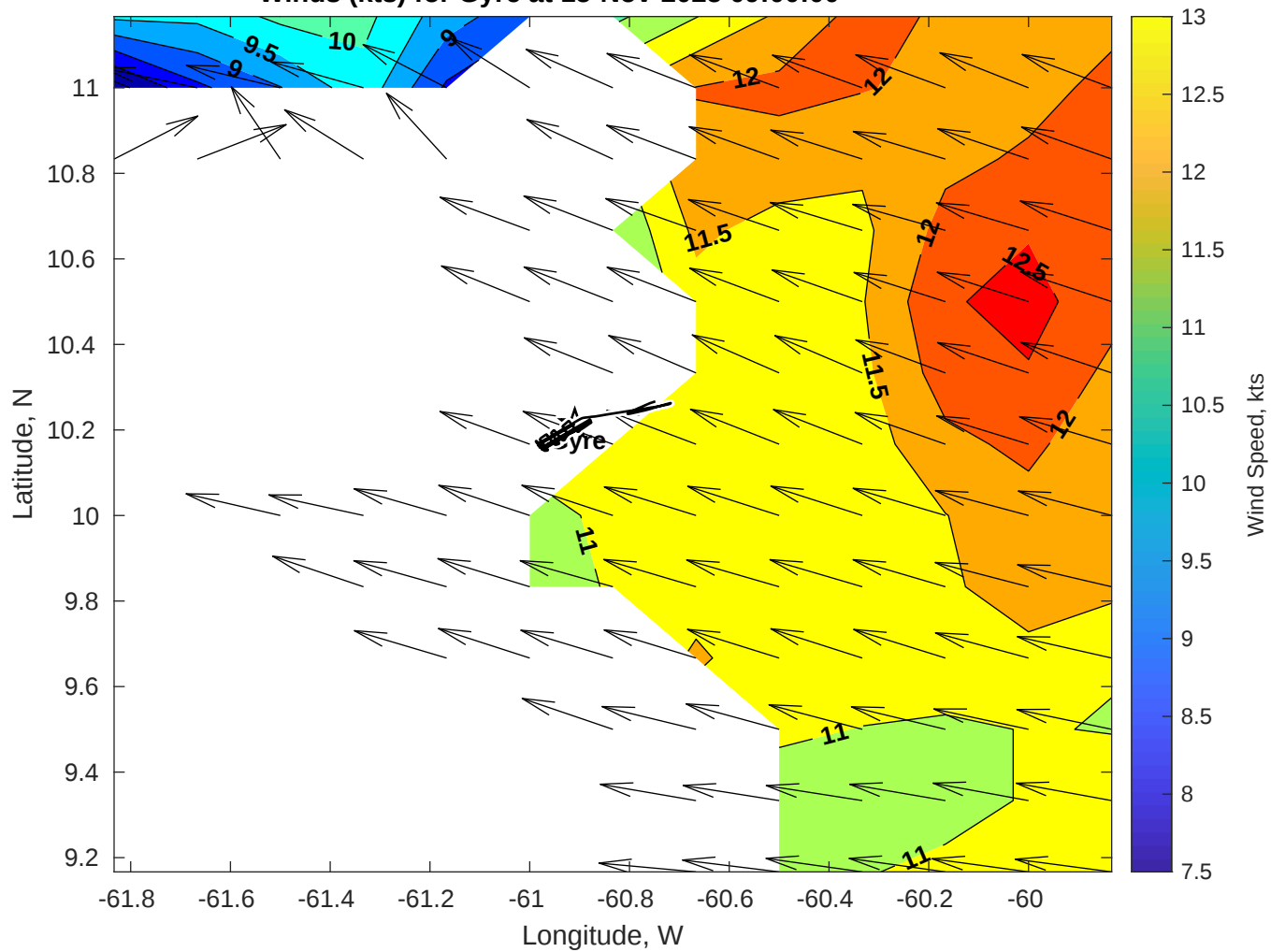
Winds (kts) for Gyre at 15-Nov-2025 09:00:00
