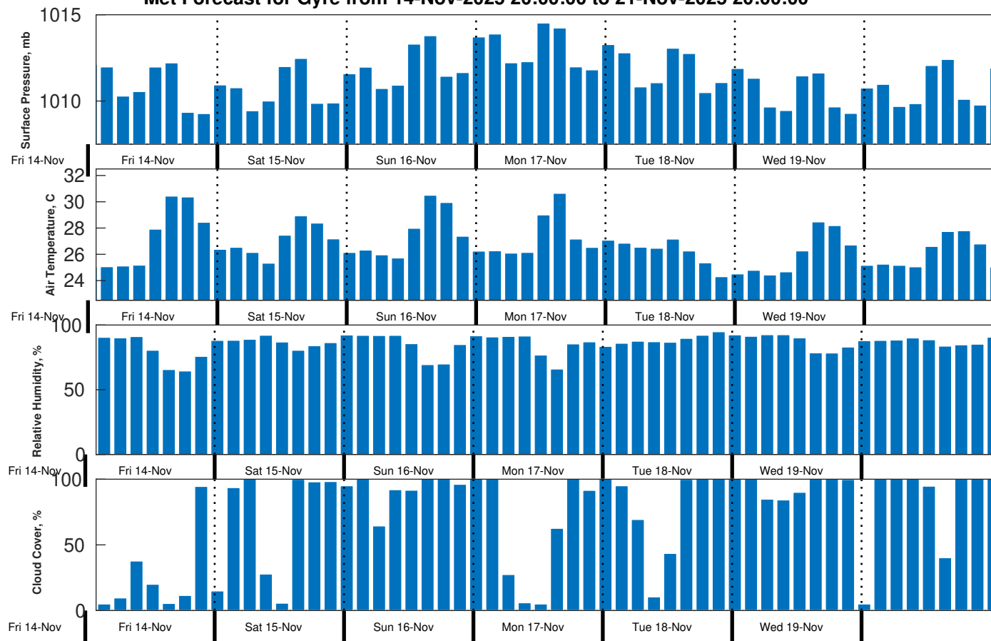
Met Forecast for Gyre from 14-Nov-2025 20:00:00 to 21-Nov-2025 20:00:00
