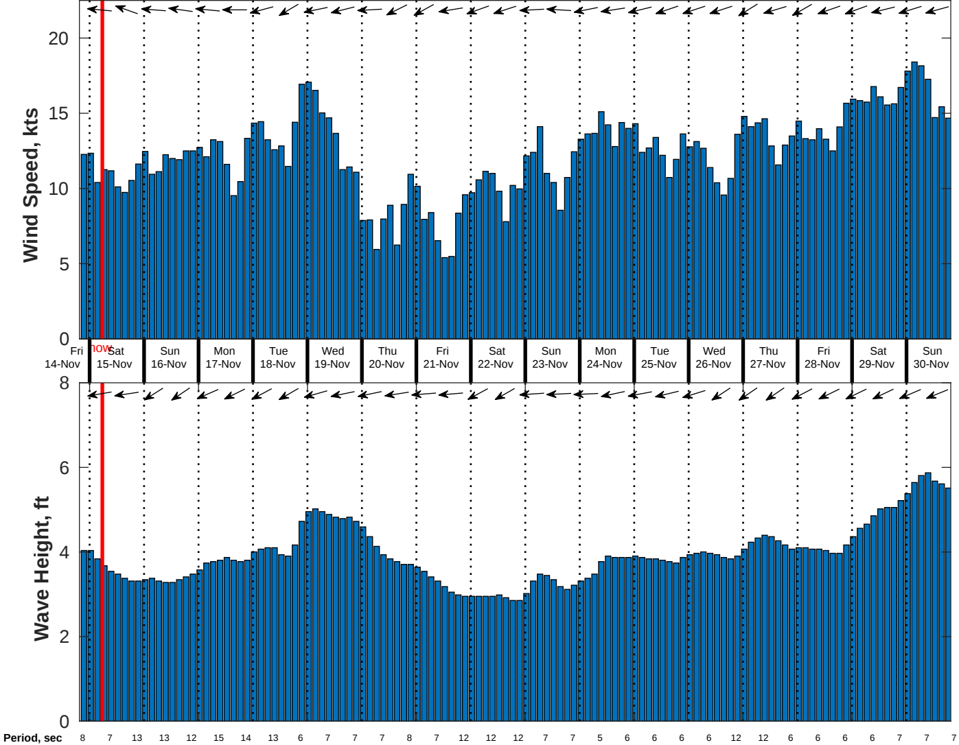
Wind & Wave Forecast for Gyre from 14-Nov-2025 20:00:00 to 30-Nov-2025 20:00:00
