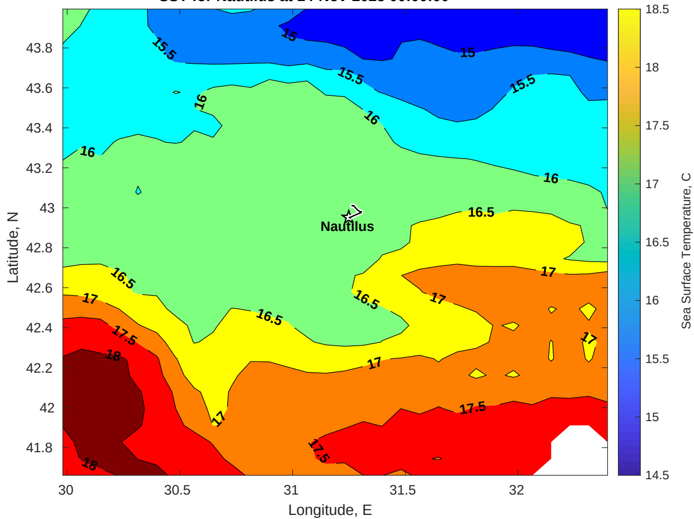
SST for Nautilus at 14-Nov-2025 00:00:00
