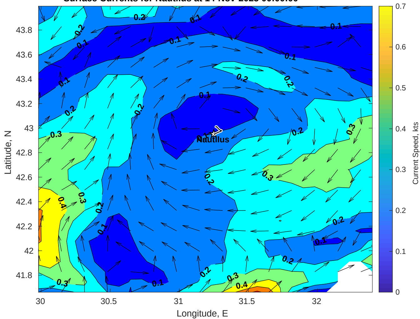
Surface Currents for Nautilus at 14-Nov-2025 00:00:00
