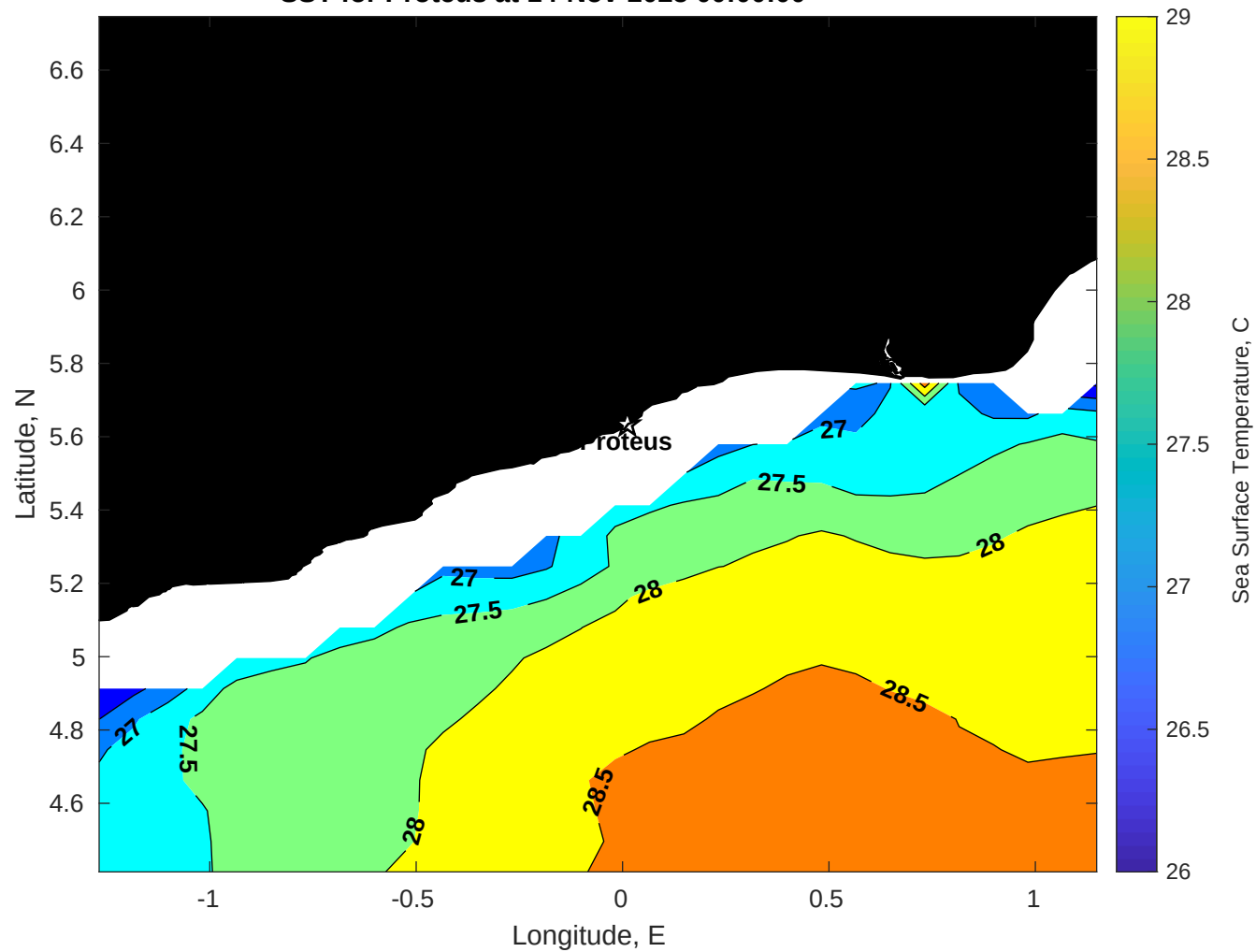
SST for Proteus at 14-Nov-2025 00:00:00
