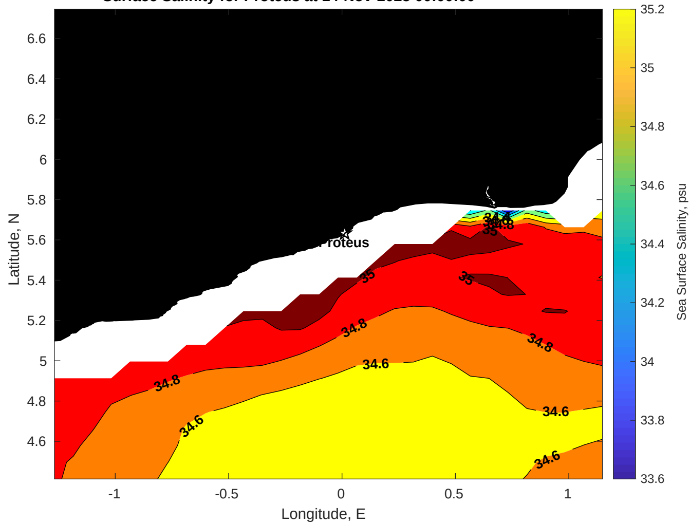
Surface Salinity for Proteus at 14-Nov-2025 00:00:00
