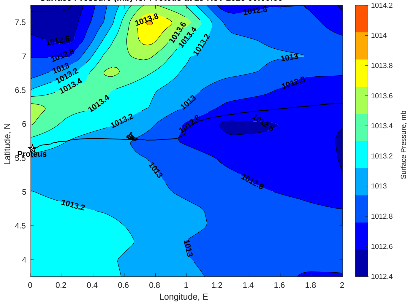
Surface Pressure (mb) for Proteus at 15-Nov-2025 00:00:00
