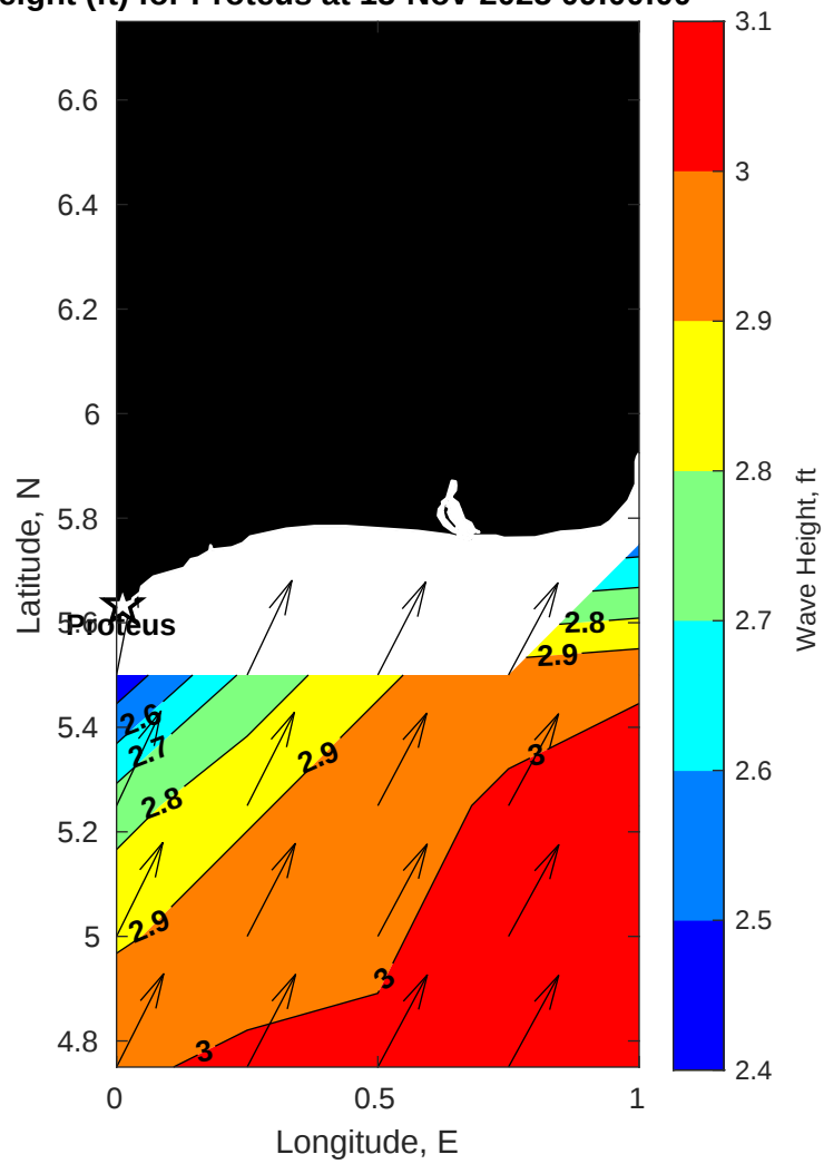
Wave Height (ft) for Proteus at 15-Nov-2025 09:00:00
