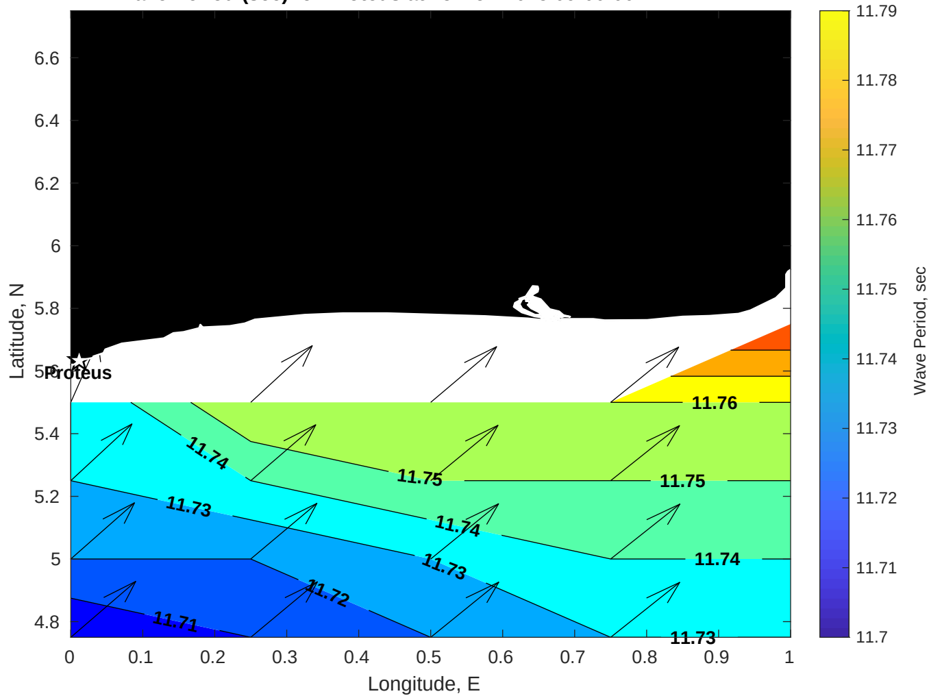
Wave Period (sec) for Proteus at 15-Nov-2025 09:00:00
