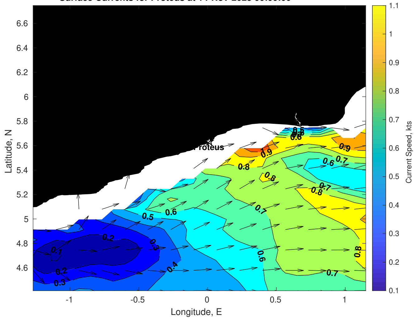
Surface Currents for Proteus at 14-Nov-2025 00:00:00
