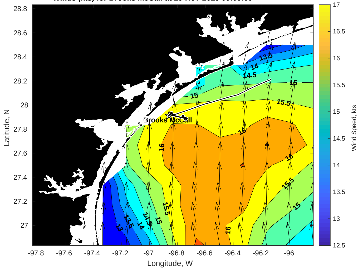
Winds (kts) for Brooks McCall at 16-Nov-2025 09:00:00
