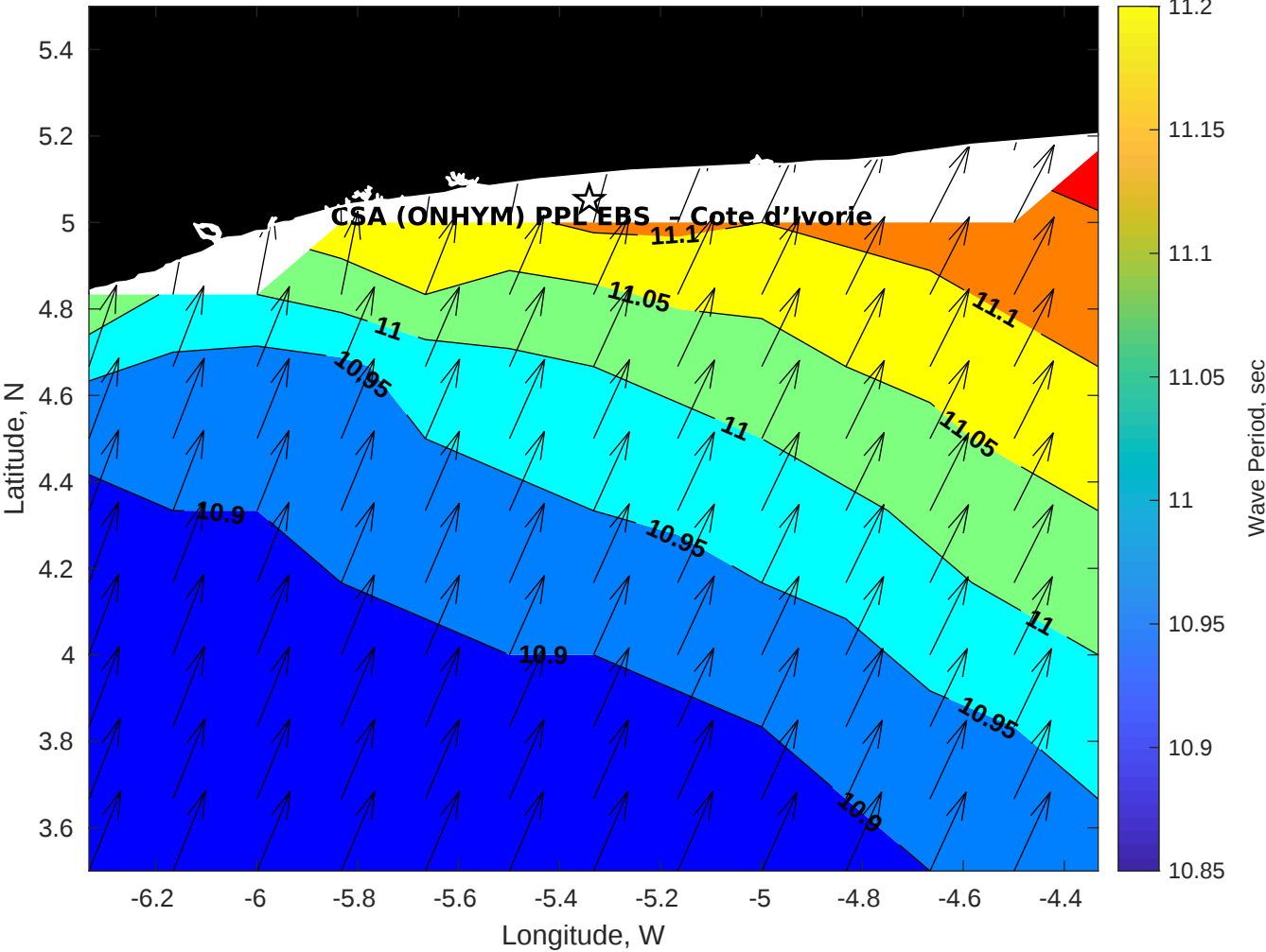
Wave Period (sec) for CSA (ONHYM) PPL EBS - Cote d'Ivoire at 16-Nov-2025 09:00:00
