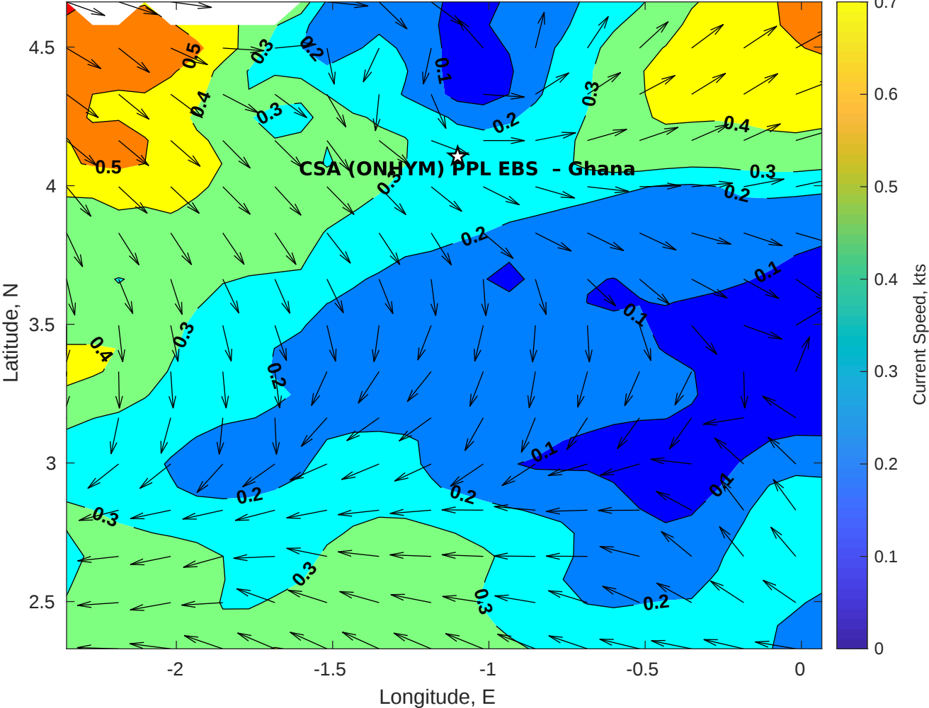
Surface Currents for CSA (ONHYM) PPL EBS - Ghana at 15-Nov-2025 00:00:00
