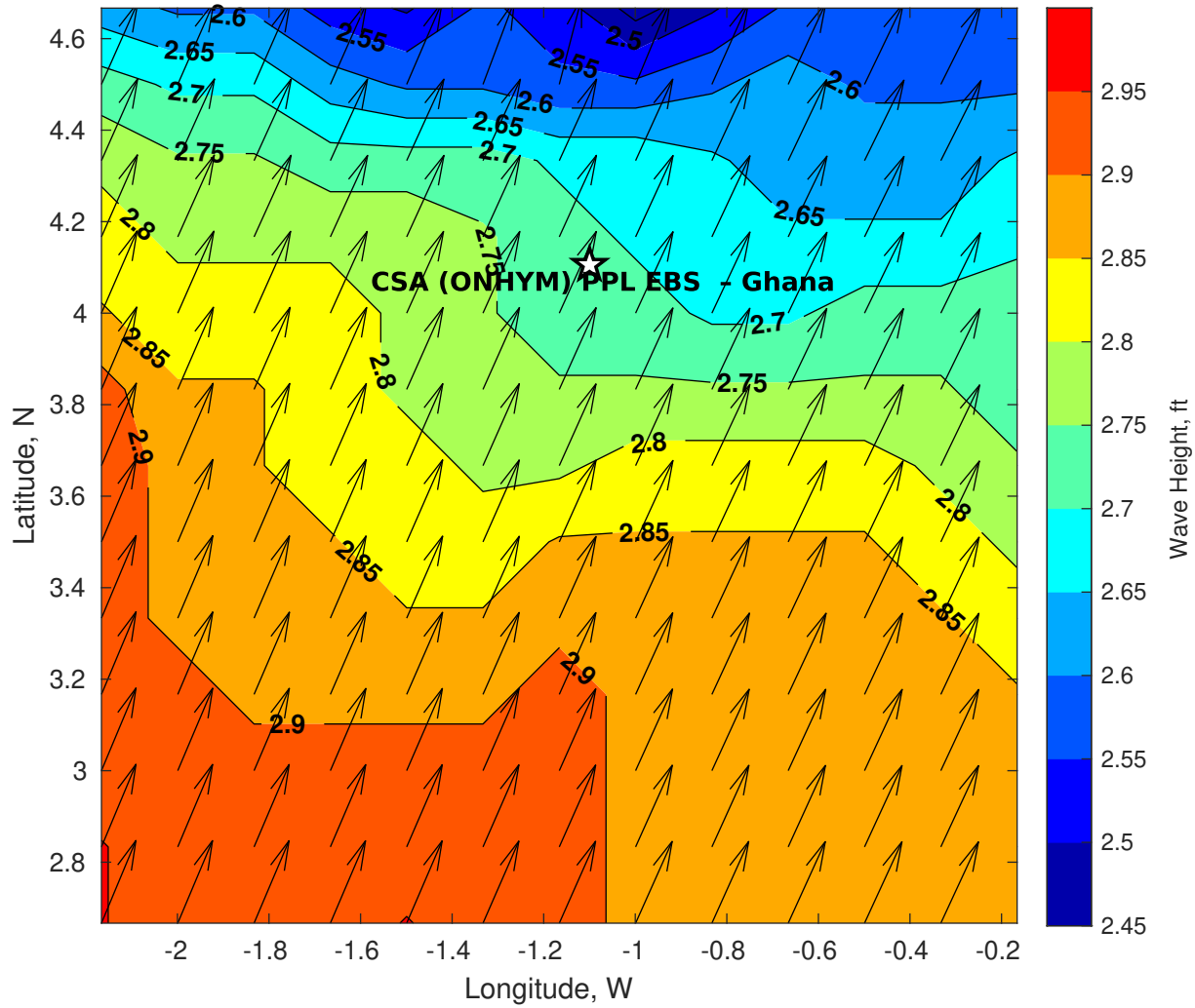
Wave Height (ft) for CSA (ONHYM) PPL EBS - Ghana at 16-Nov-2025 09:00:00
