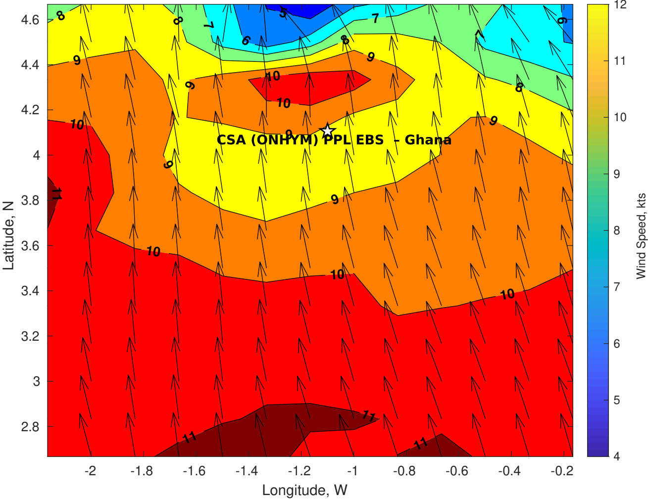
Winds (kts) for CSA (ONHYM) PPL EBS - Ghana at 16-Nov-2025 09:00:00
