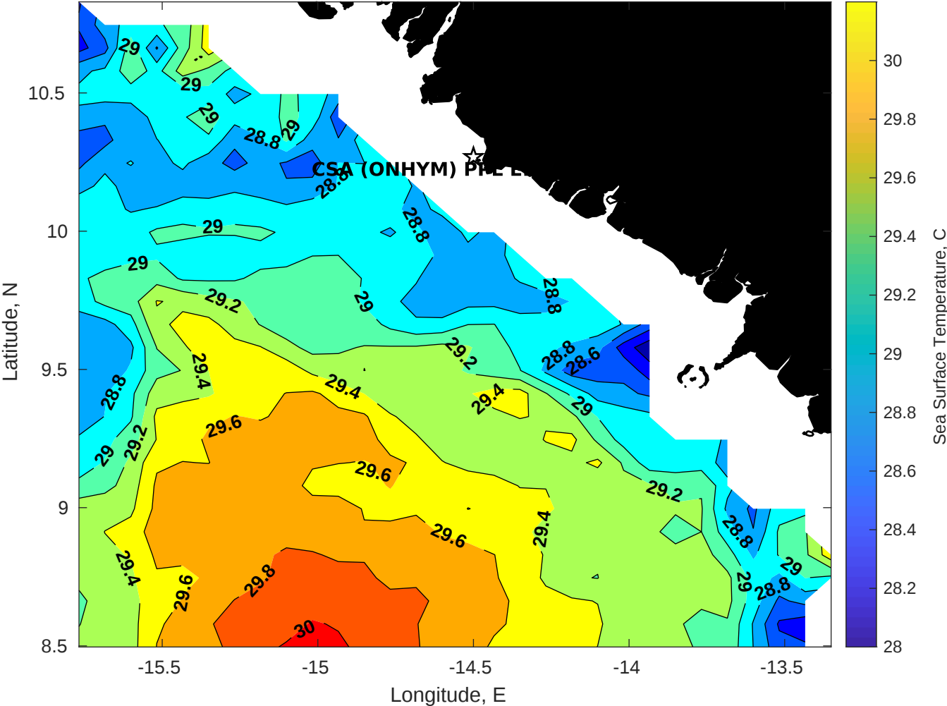
SST for CSA (ONHYM) PPL EBS - Guinea at 15-Nov-2025 00:00:00
