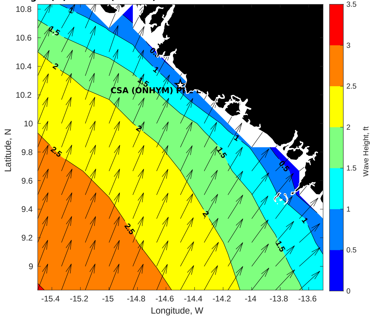
Wave Height (ft) for CSA (ONHYM) PPL EBS - Guinea at 16-Nov-2025 09:00:00
