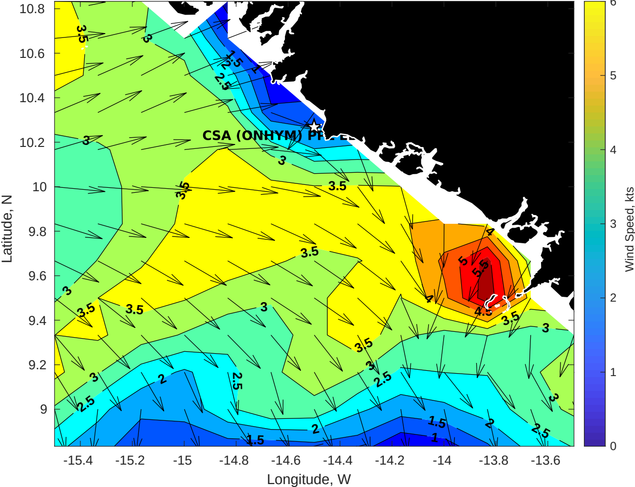
Winds (kts) for CSA (ONHYM) PPL EBS - Guinea at 16-Nov-2025 09:00:00
