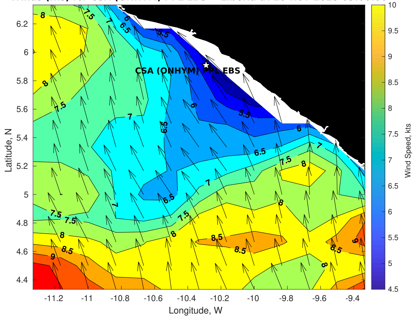
Winds (kts) for CSA (ONHYM) PPL EBS - Liberia at 16-Nov-2025 09:00:00
