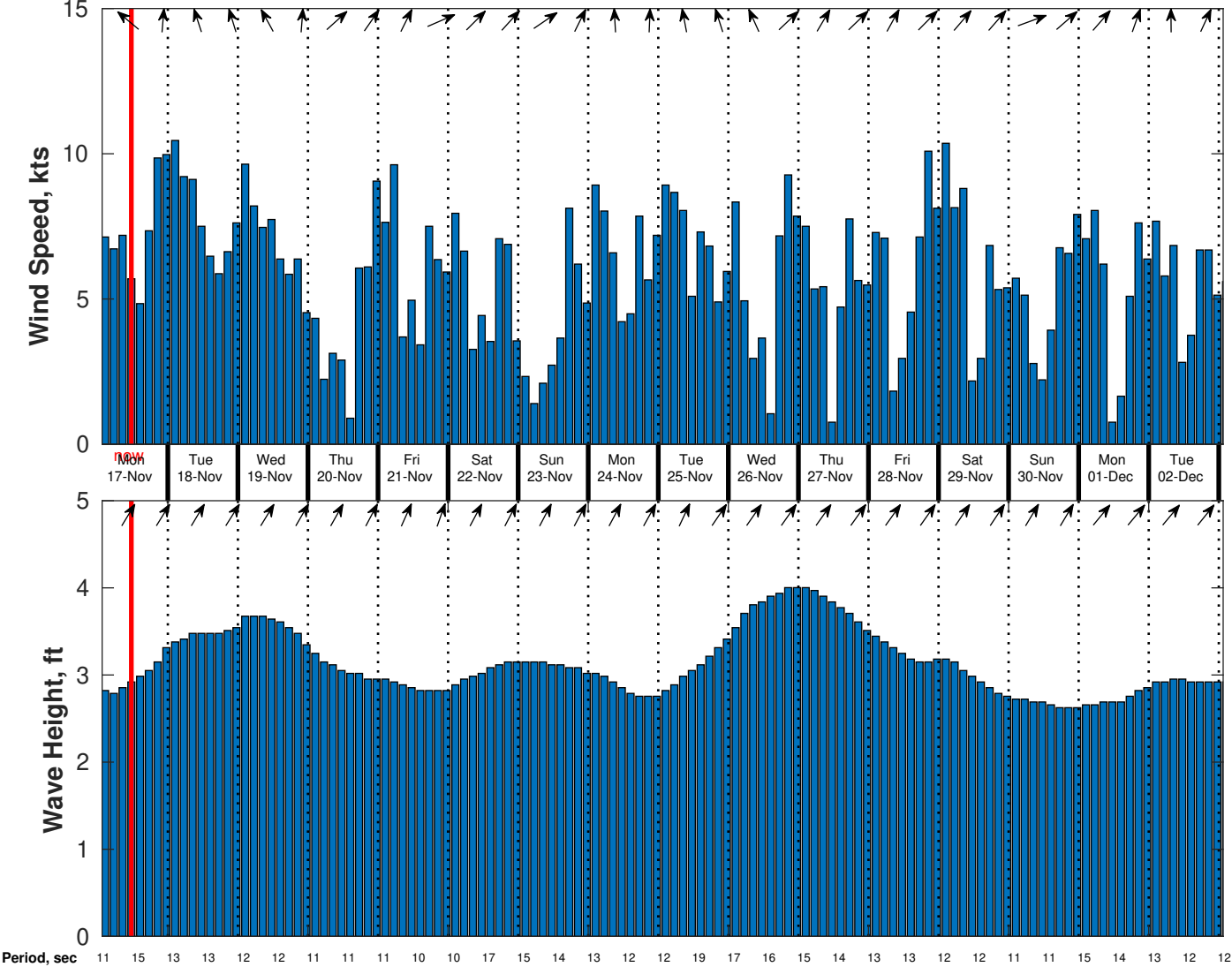
Wind & Wave Forecast for CSA (ONHYM) PPL EBS - Liberia from 16-Nov-2025 01:00:00 to 02-Dec-2025 01:00:00
