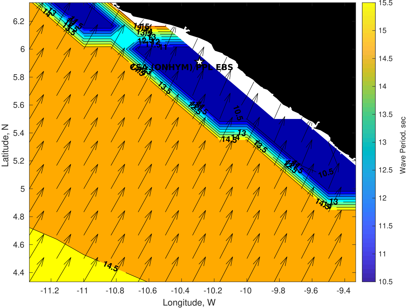
Wave Period (sec) for CSA (ONHYM) PPL EBS - Liberia at 16-Nov-2025 09:00:00
