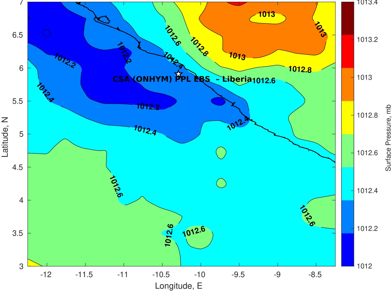
Surface Pressure (mb) for CSA (ONHYM) PPL EBS - Liberia at 18-Nov-2025 00:00:00
