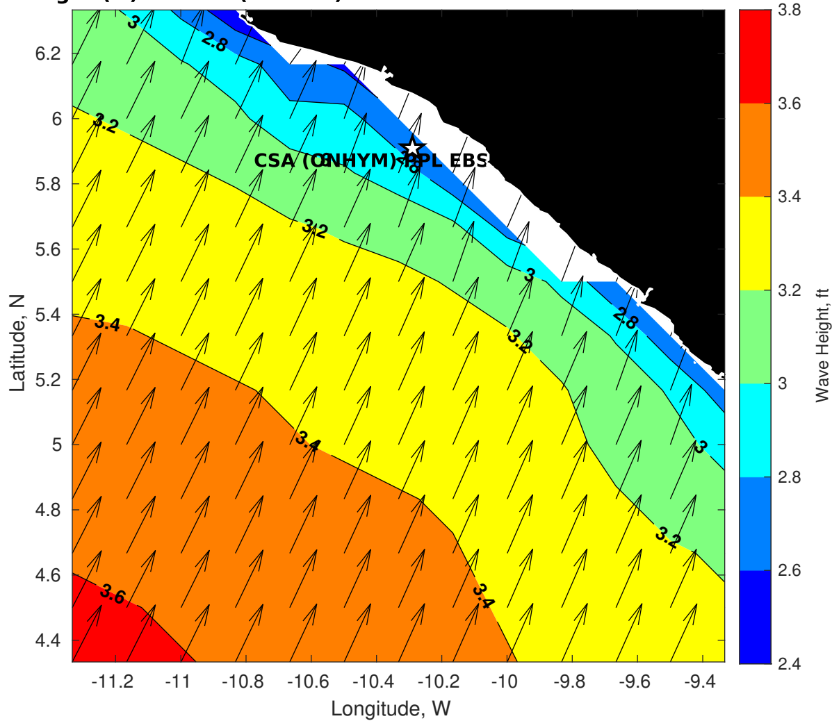
Wave Height (ft) for CSA (ONHYM) PPL EBS - Liberia at 16-Nov-2025 09:00:00
