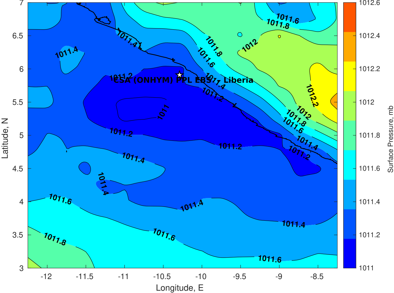
Surface Pressure (mb) for CSA (ONHYM) PPL EBS - Liberia at 16-Nov-2025 00:00:00
