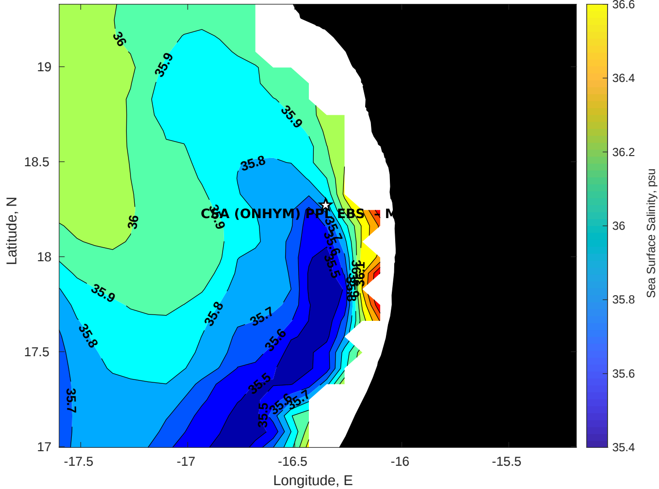
Surface Salinity for CSA (ONHYM) PPL EBS - Mauritania at 13-Nov-2025 00:00:00
