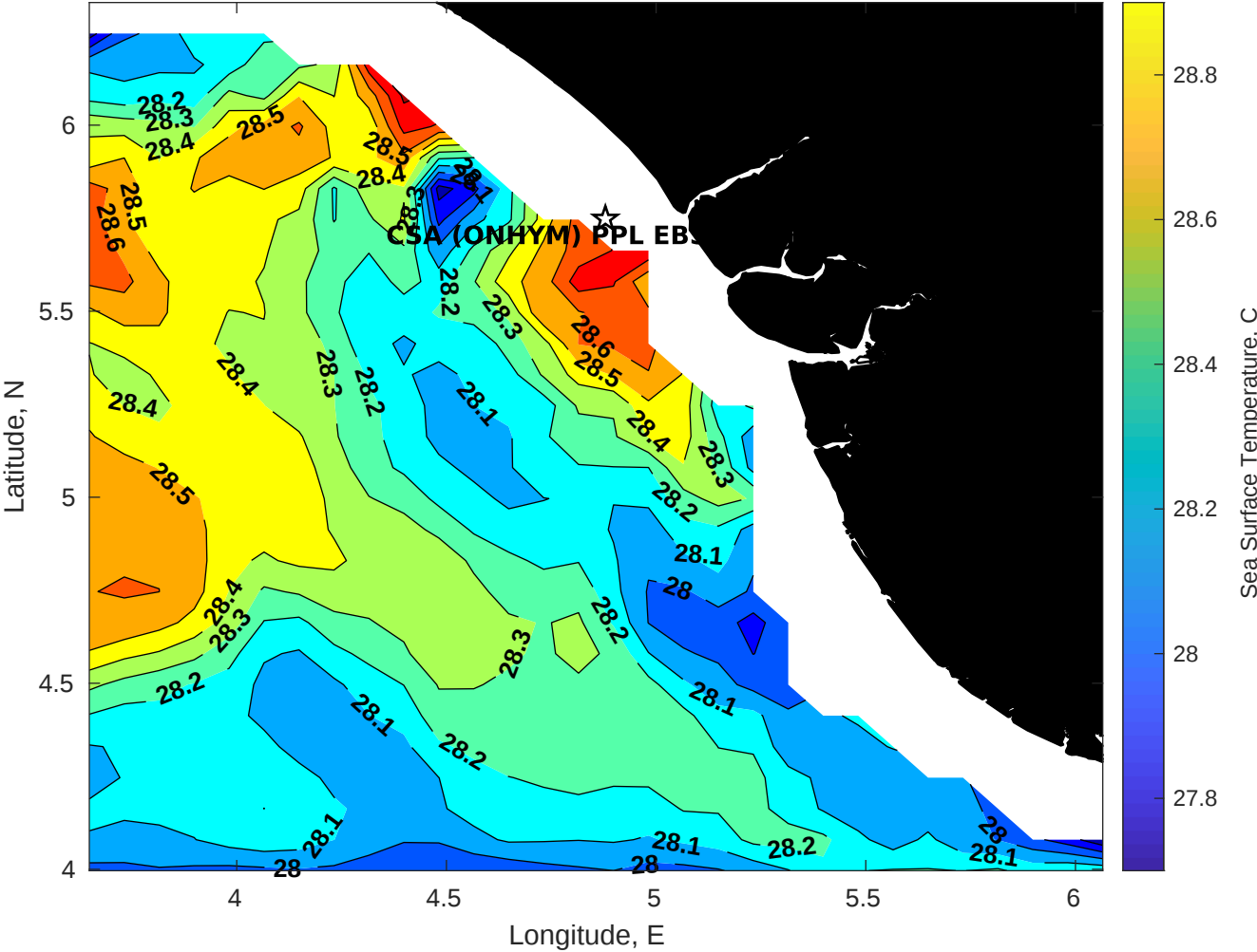
SST for CSA (ONHYM) PPL EBS - Nigeria at 15-Nov-2025 00:00:00
