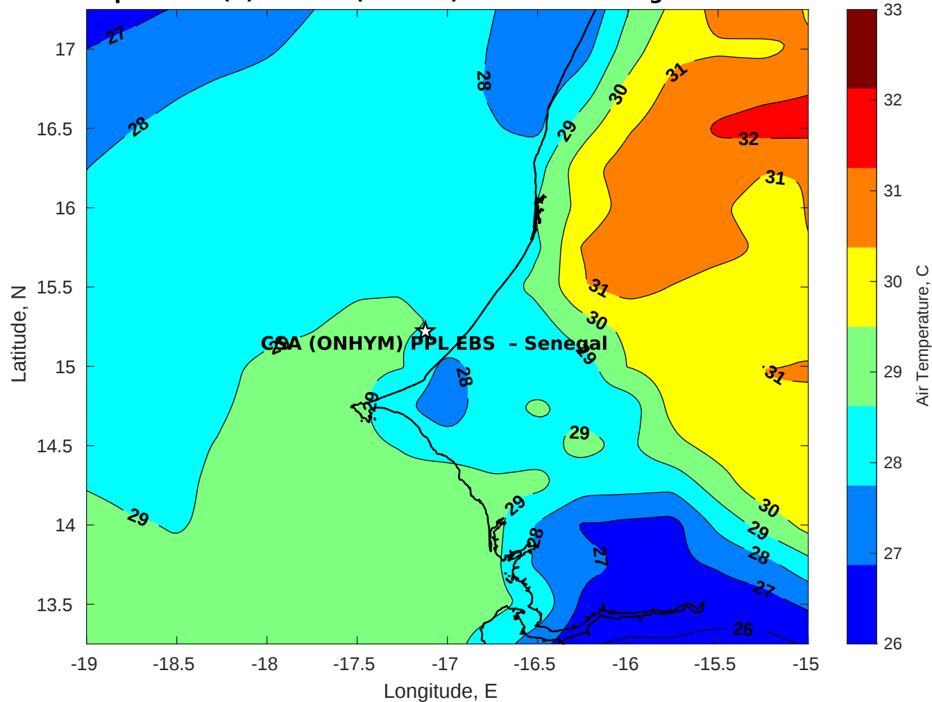
Air Temperature (C) for CSA (ONHYM) PPL EBS - Senegal at 16-Nov-2025
