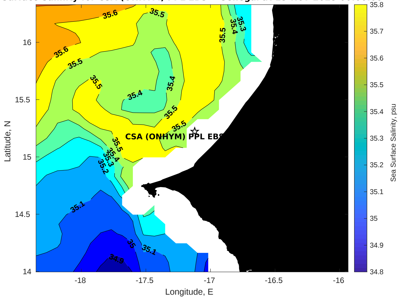
Surface Salinity for CSA (ONHYM) PPL EBS - Senegal at 15-Nov-2025 00:00:00
