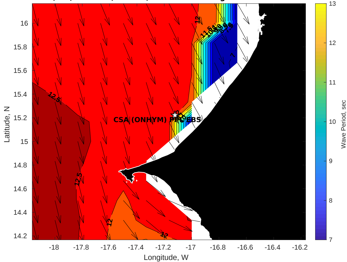
Wave Period (sec) for CSA (ONHYM) PPL EBS - Senegal at 16-Nov-2025 09:00:00
