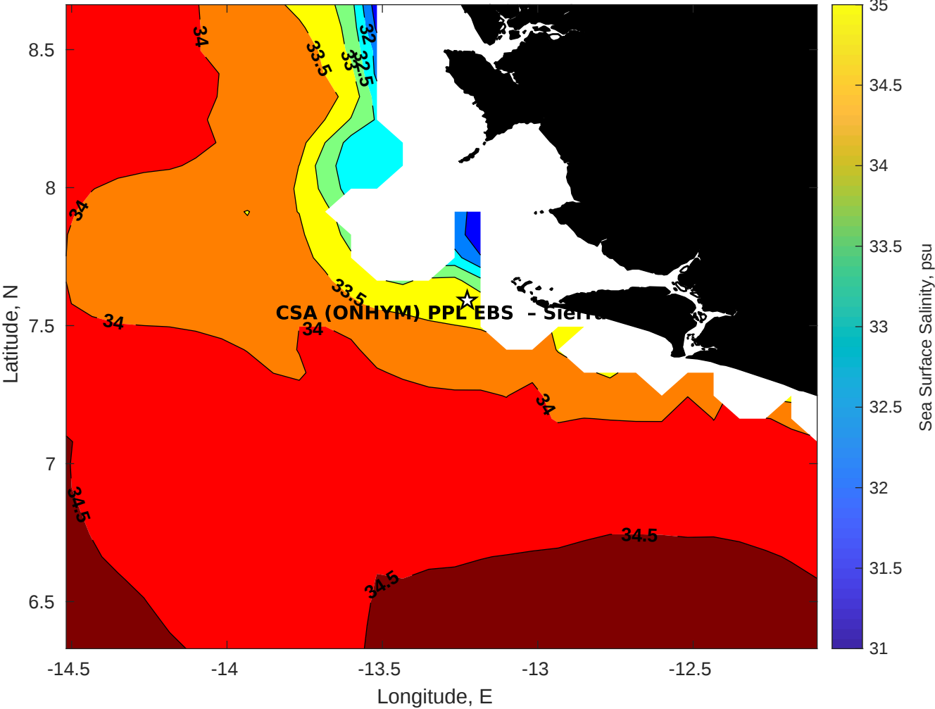
Surface Salinity for CSA (ONHYM) PPL EBS - Sierra Leone at 15-Nov-2025 00:00:00
