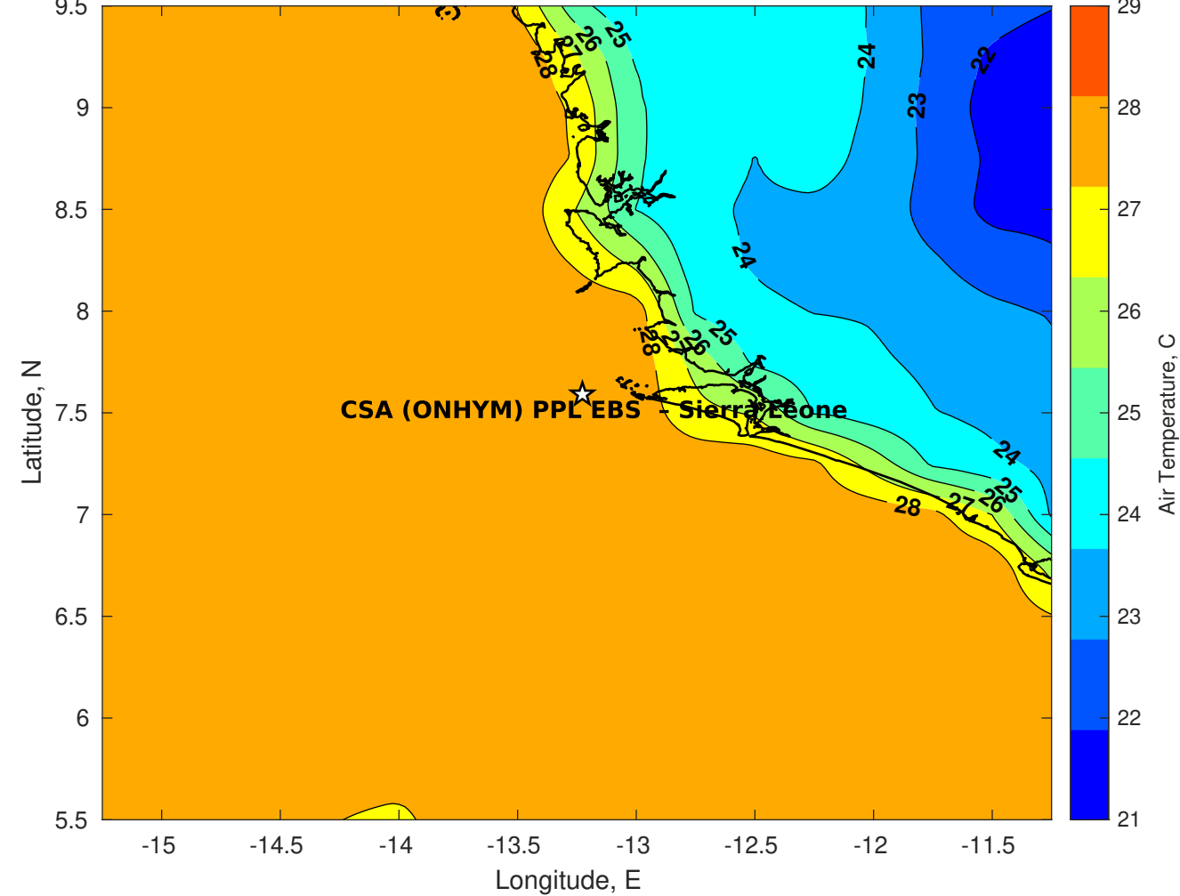
Air Temperature (C) for CSA (ONHYM) PPL EBS - Sierra Leone at 16-Nov-2025
