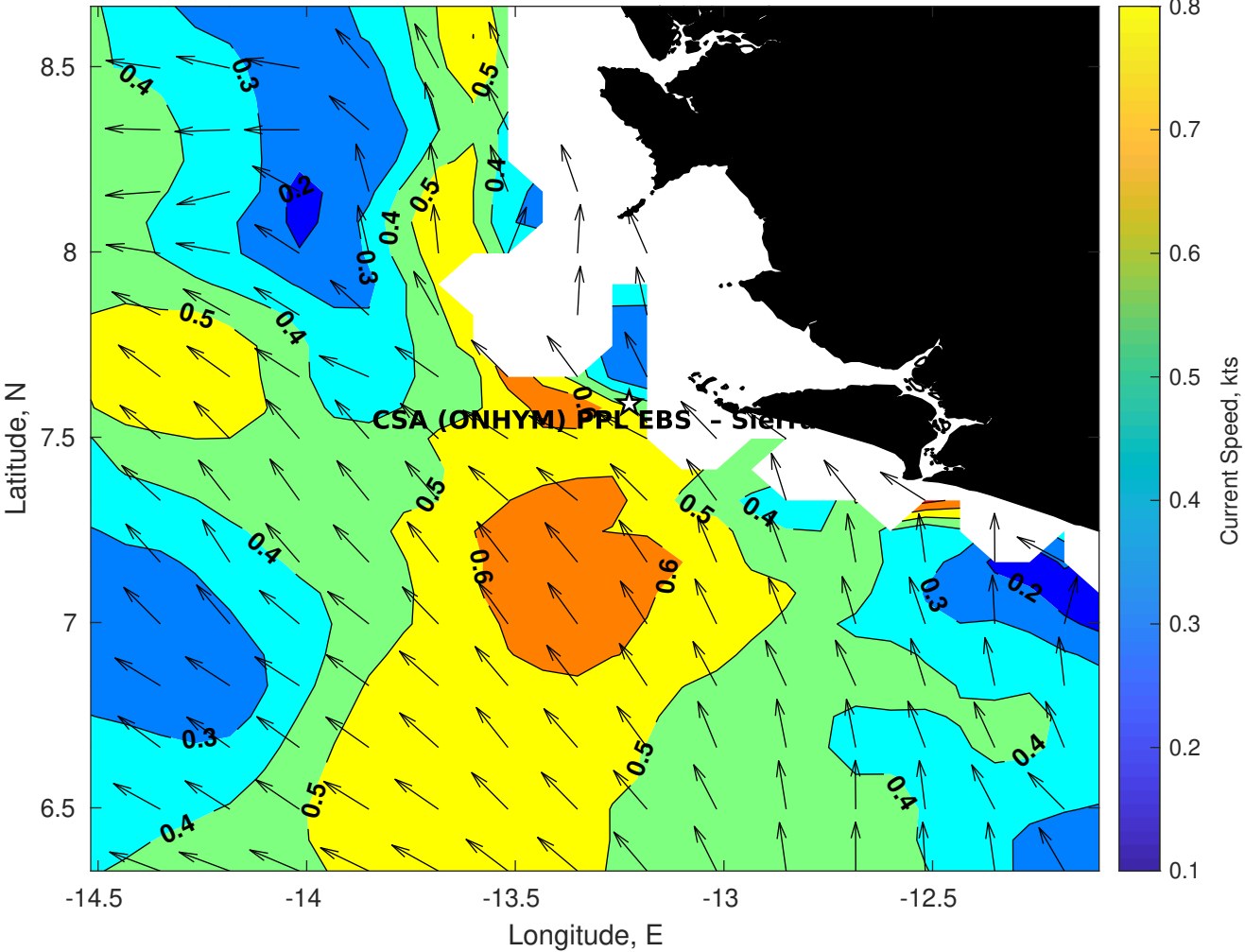
Surface Currents for CSA (ONHYM) PPL EBS - Sierra Leone at 15-Nov-2025 00:00:00
