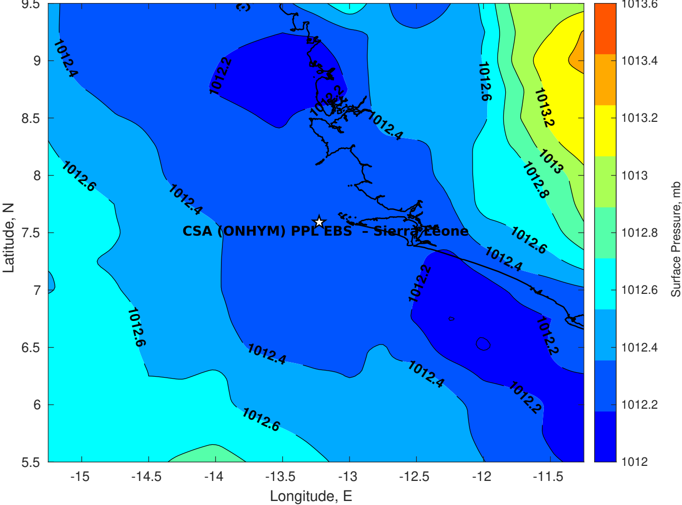
Surface Pressure (mb) for CSA (ONHYM) PPL EBS - Sierra Leone at 18-Nov-2025 00:00:00
