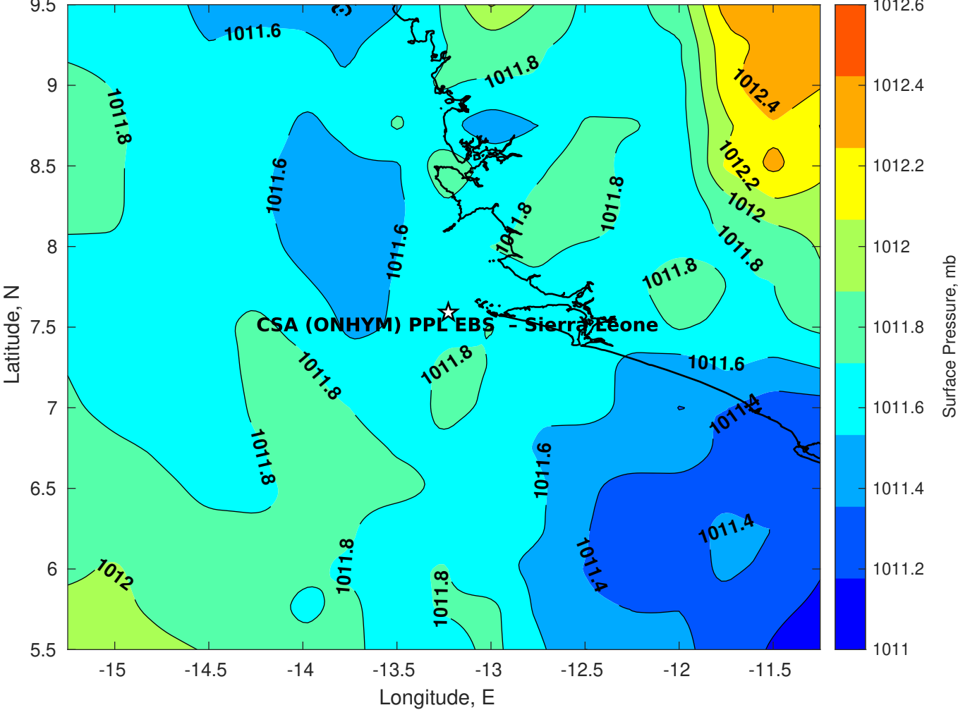
Surface Pressure (mb) for CSA (ONHYM) PPL EBS - Sierra Leone at 16-Nov-2025 00:00:00
