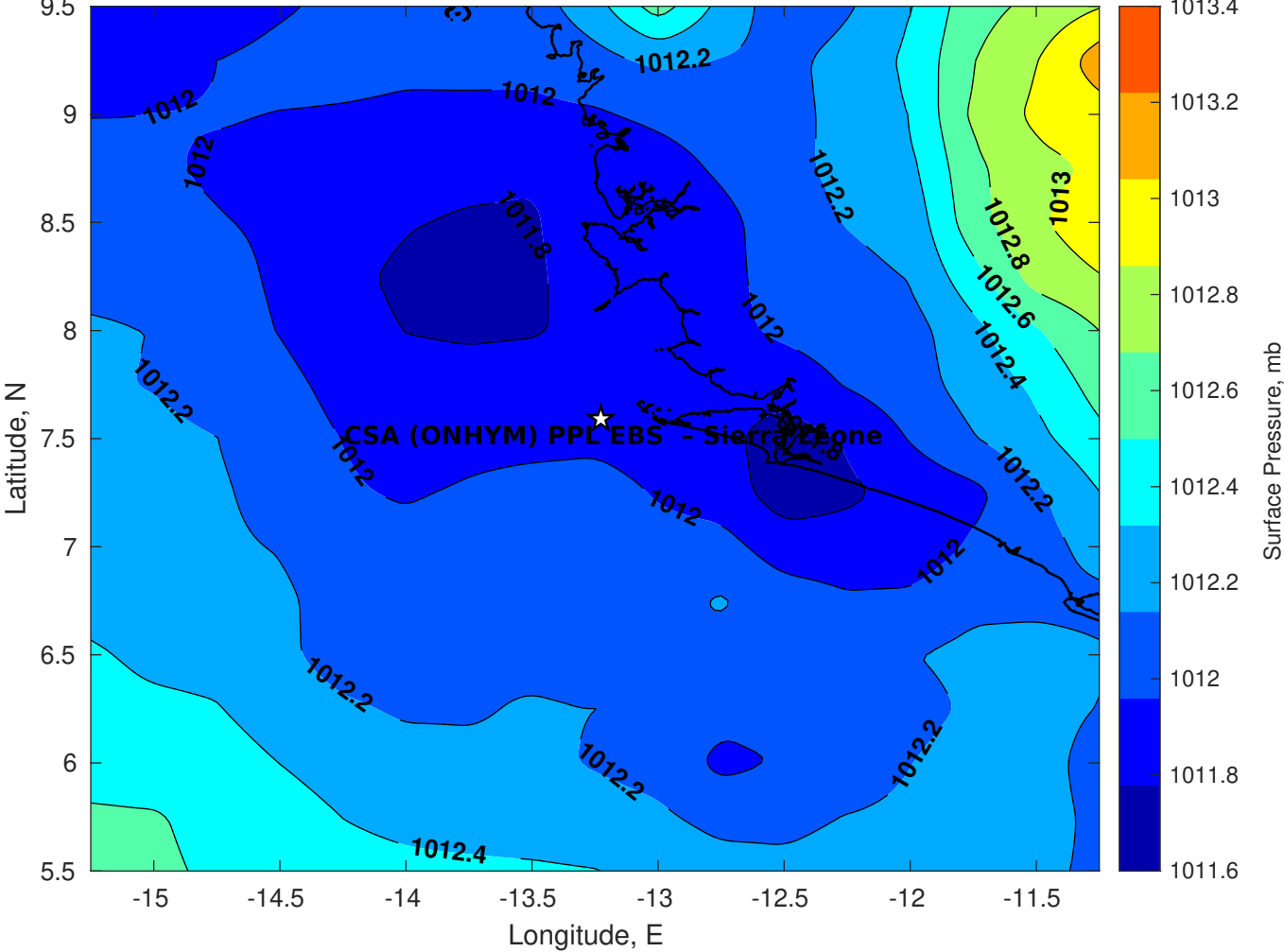
Surface Pressure (mb) for CSA (ONHYM) PPL EBS - Sierra Leone at 17-Nov-2025 00:00:00
