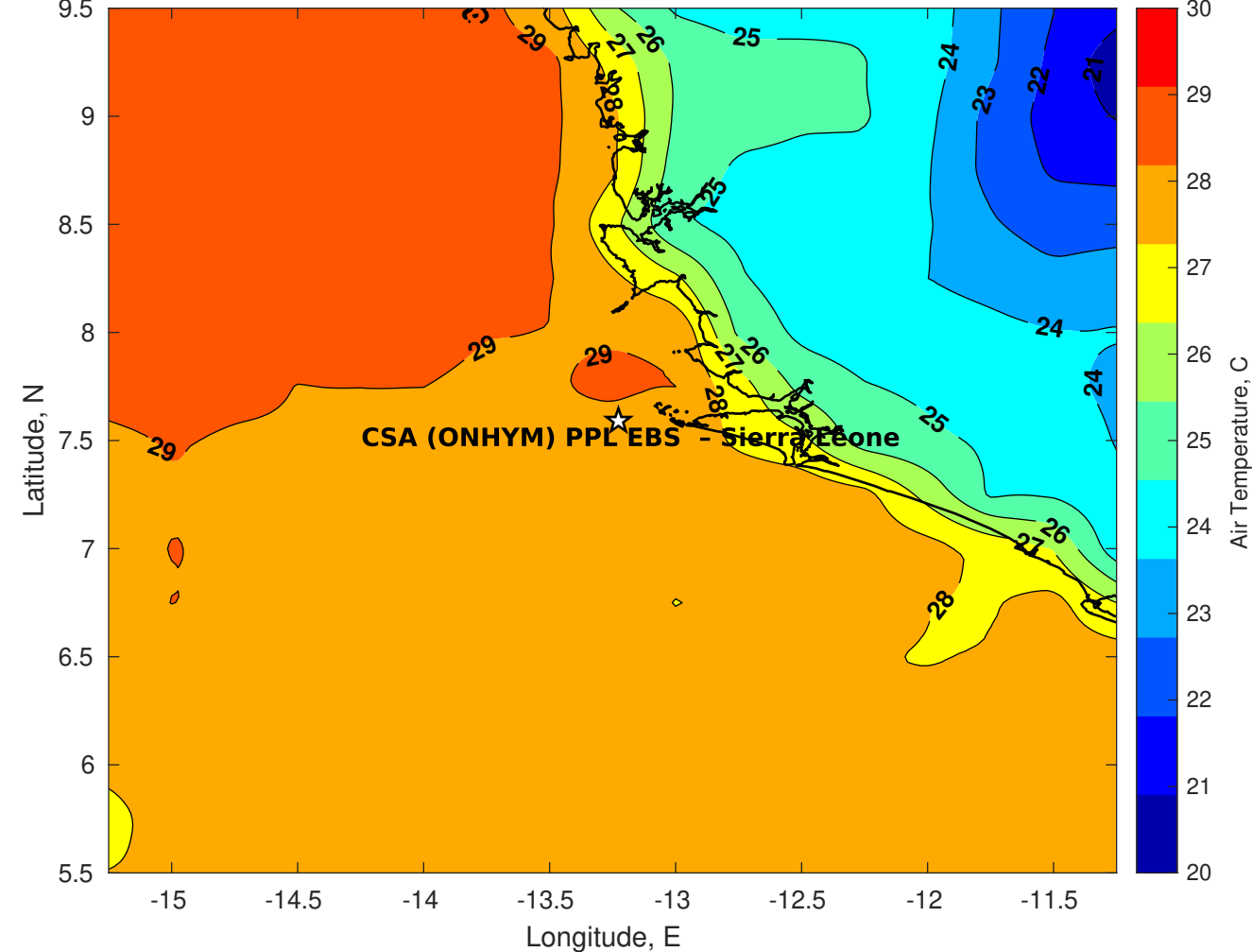
Air Temperature (C) for CSA (ONHYM) PPL EBS - Sierra Leone at 16-Nov-2025
