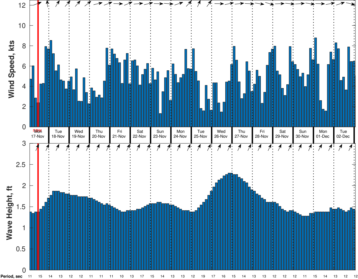
Wind & Wave Forecast for CSA (ONHYM) PPL EBS - Sierra Leone from 16-Nov-2025 01:00:00 to 02-Dec-2025 01:00:00
