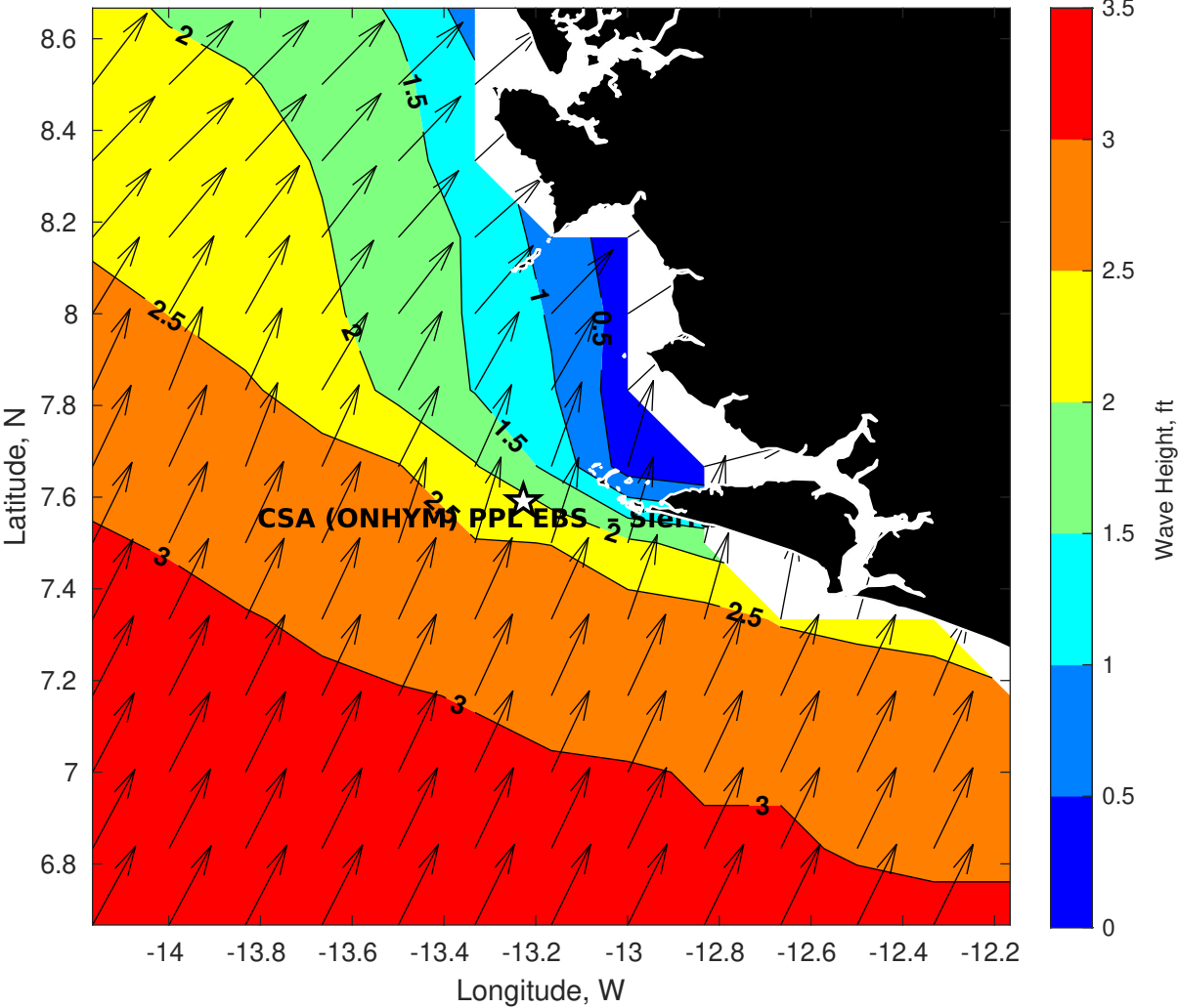
Wave Height (ft) for CSA (ONHYM) PPL EBS - Sierra Leone at 16-Nov-2025 09:00:00
