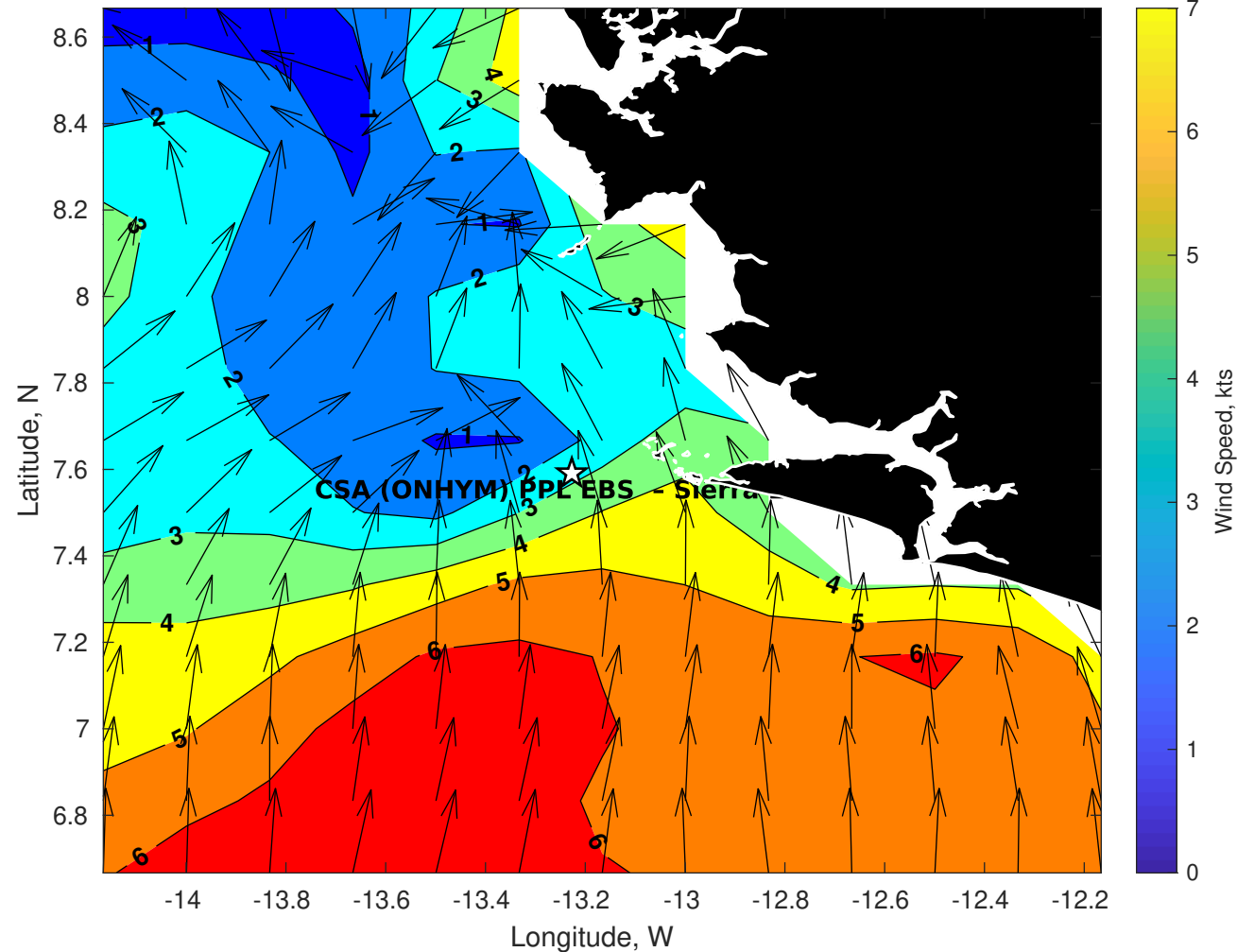
Winds (kts) for CSA (ONHYM) PPL EBS - Sierra Leone at 16-Nov-2025 09:00:00
