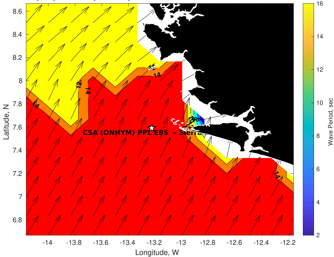
Wave Period (sec) for CSA (ONHYM) PPL EBS - Sierra Leone at 16-Nov-2025 09:00:00
