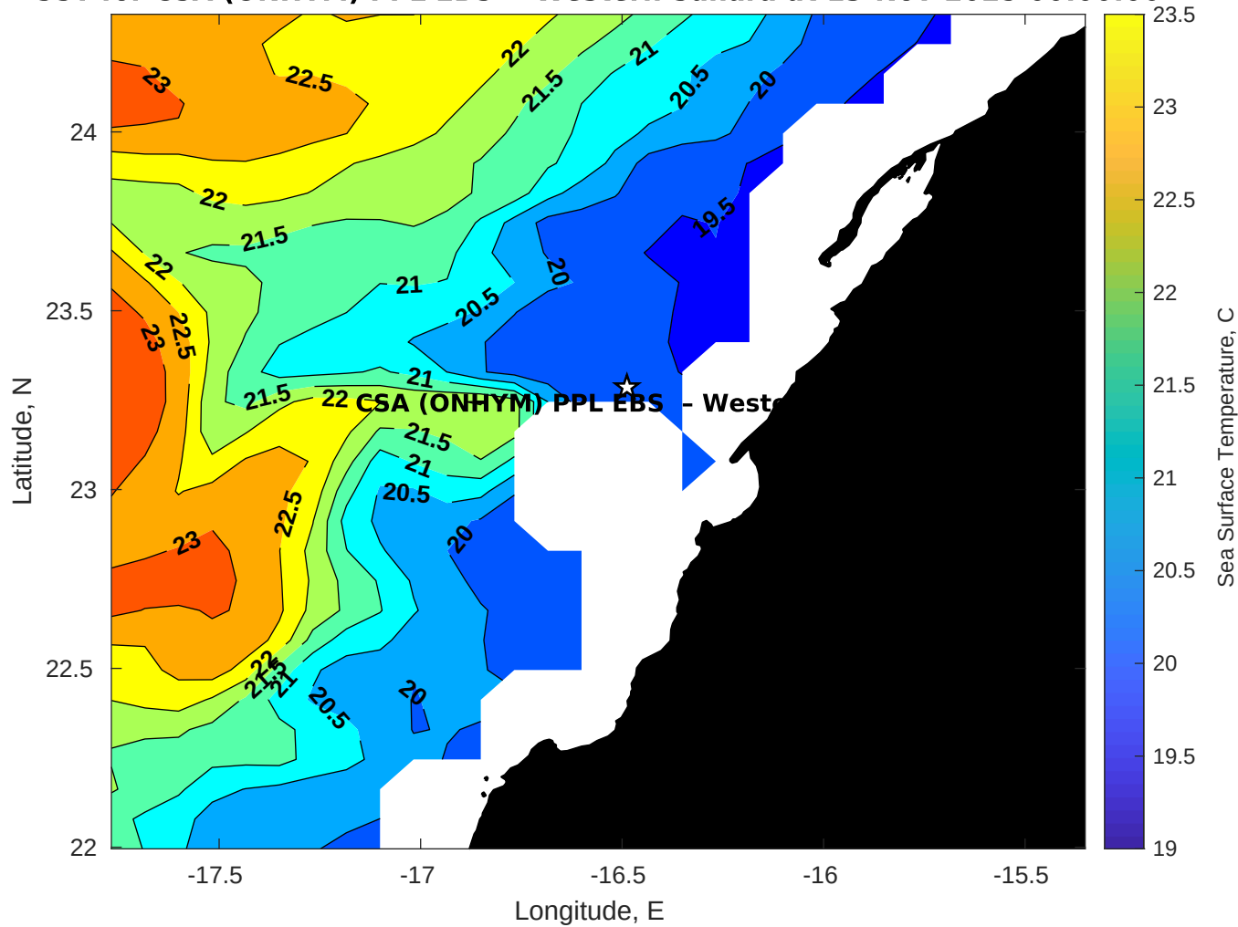
SST for CSA (ONHYM) PPL EBS - Western Sahara at 13-Nov-2025 00:00:00
