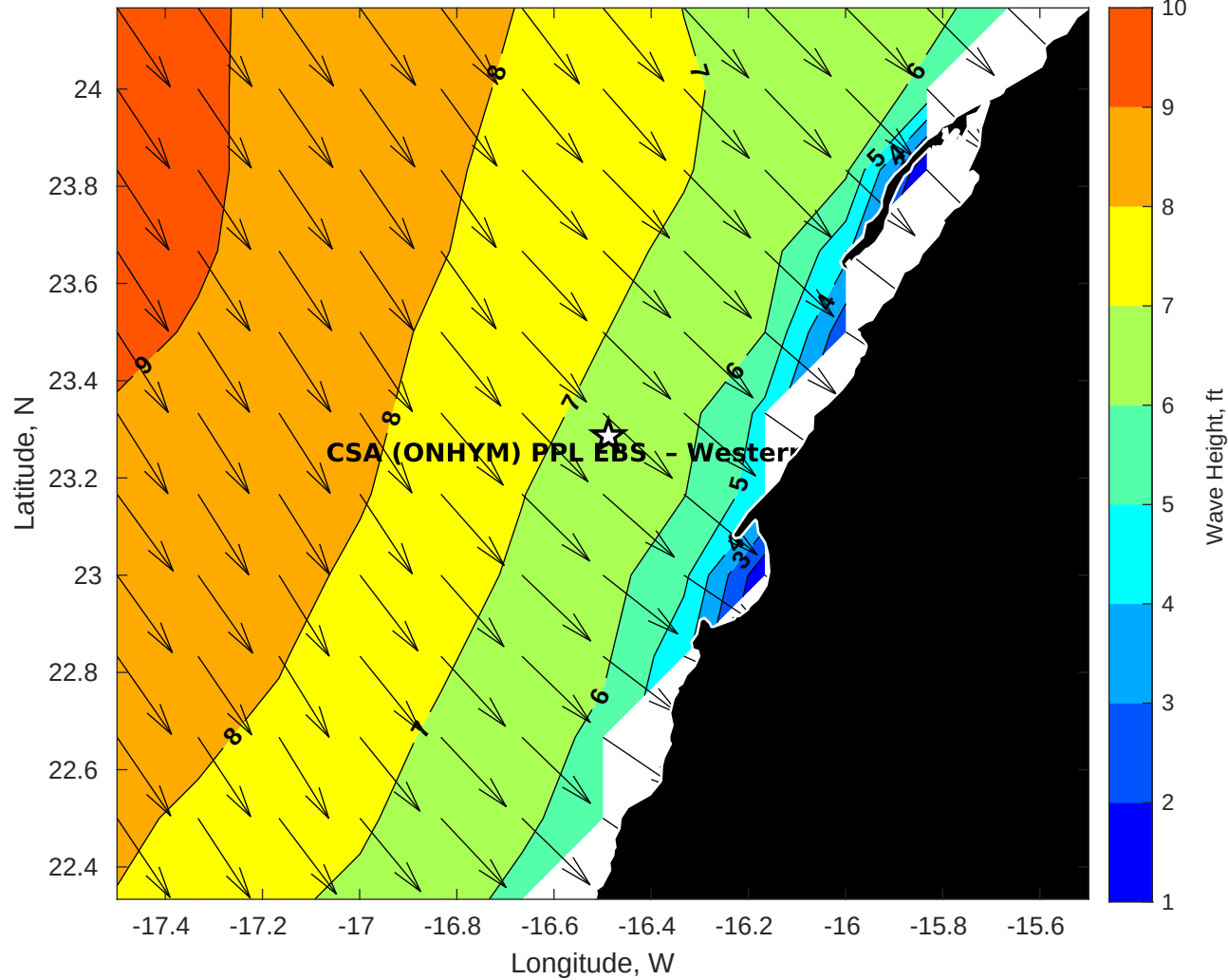
Wave Height (ft) for CSA (ONHYM) PPL EBS - Western Sahara at 14-Nov-2025 09:00:00
