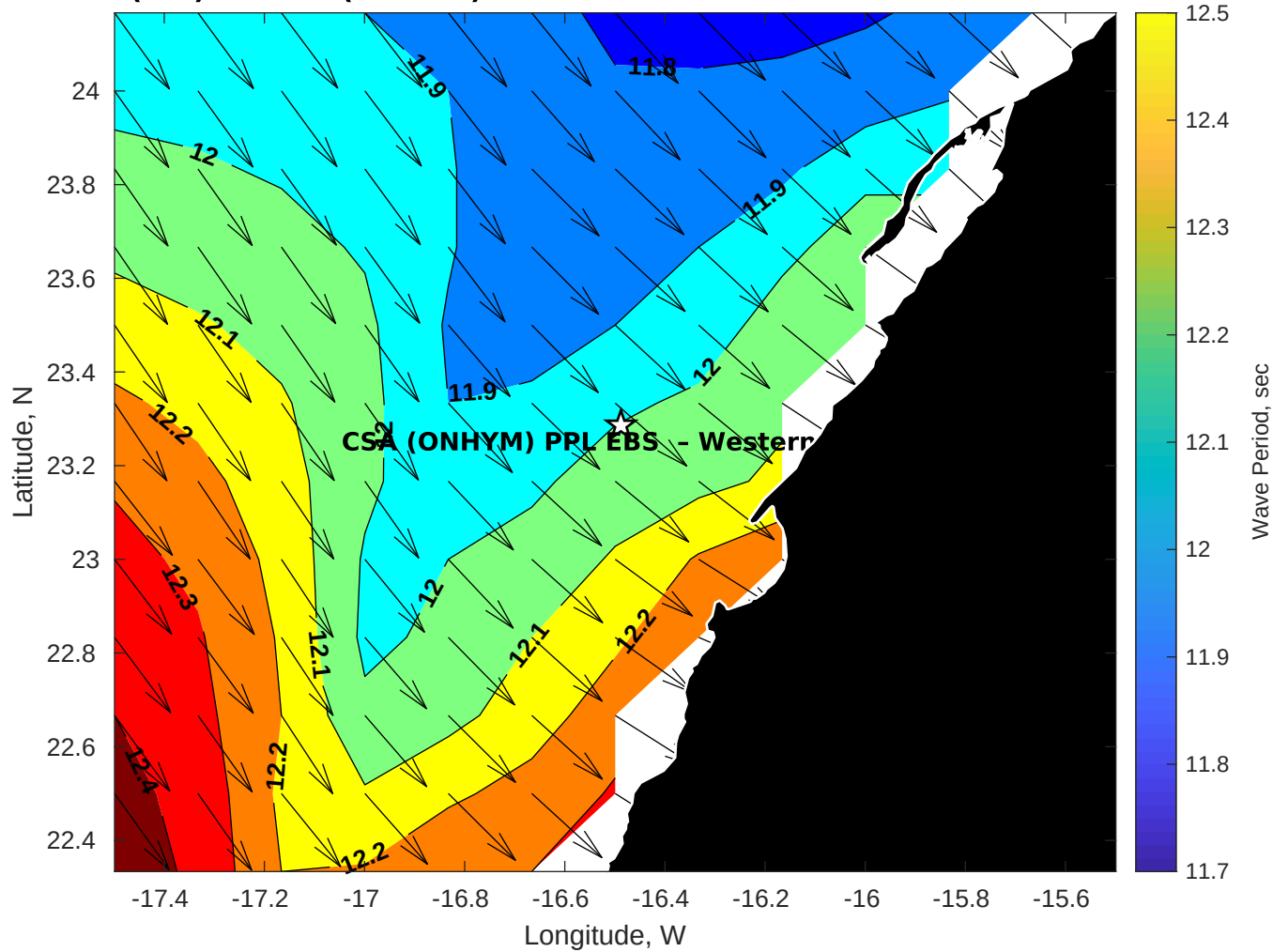
Wave Period (sec) for CSA (ONHYM) PPL EBS - Western Sahara at 14-Nov-2025 09:00:00
