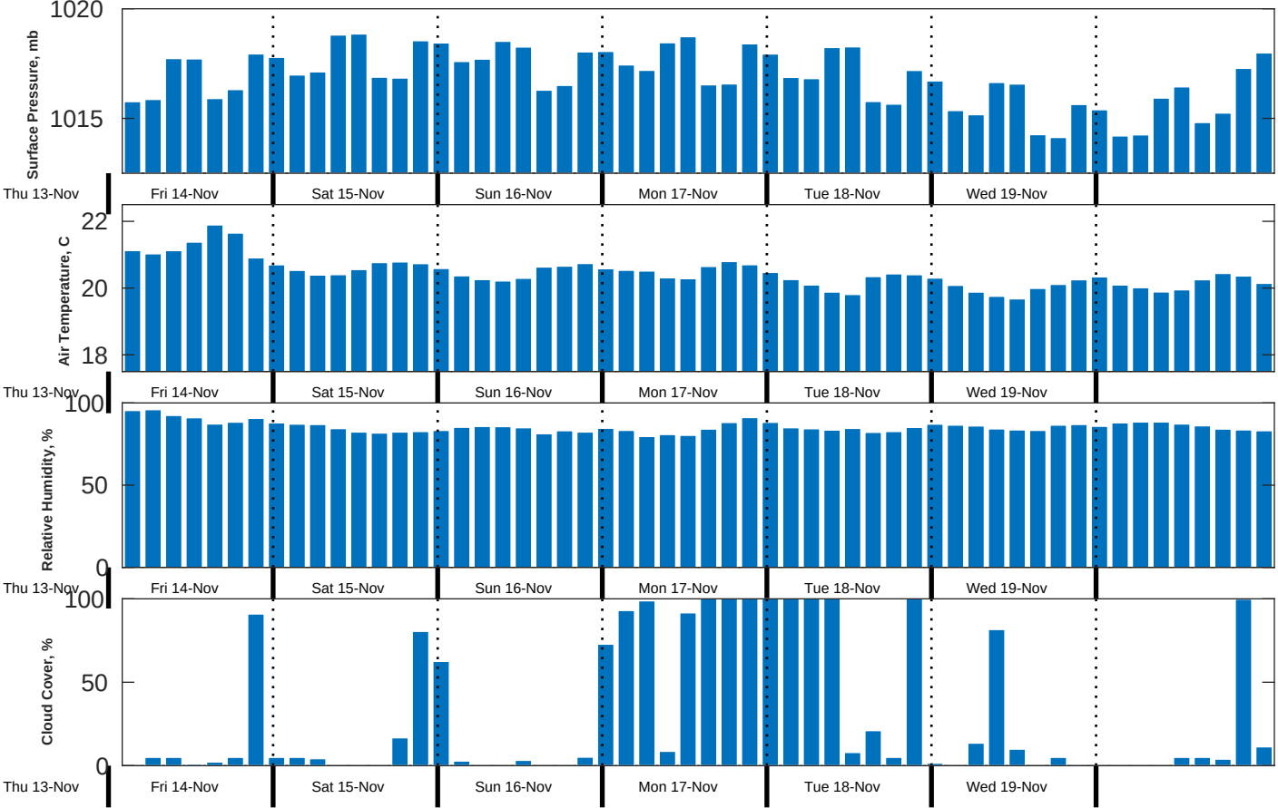
Met Forecast for CSA (ONHYM) PPL EBS - Western Sahara from 14-Nov-2025 00:00:00 to 21-Nov-2025 00:00:00
