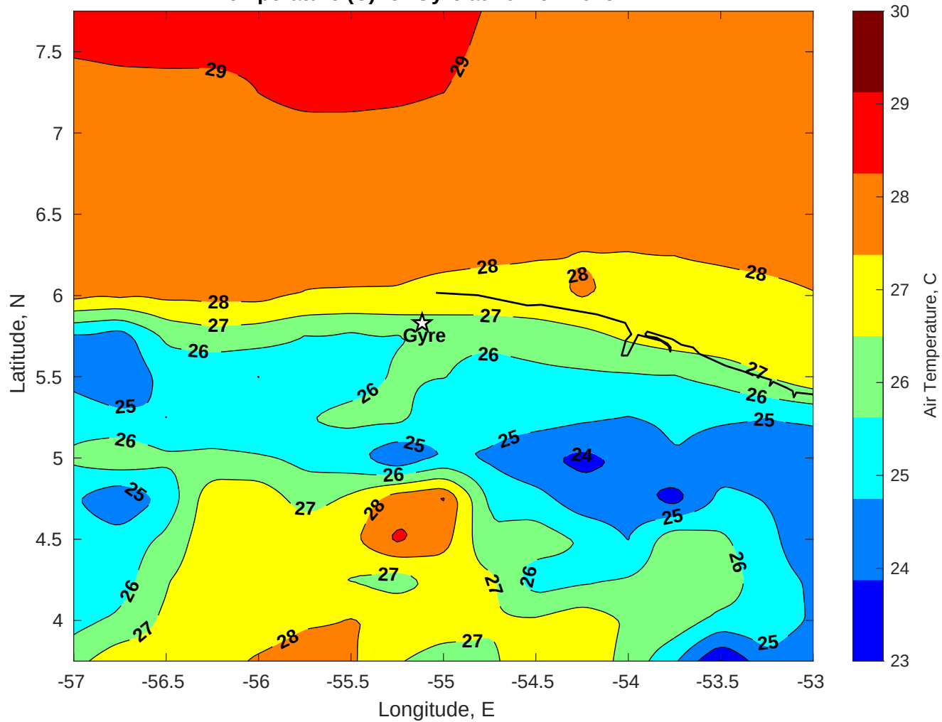
Air Temperature (C) for Gyre at 16-Nov-2025
