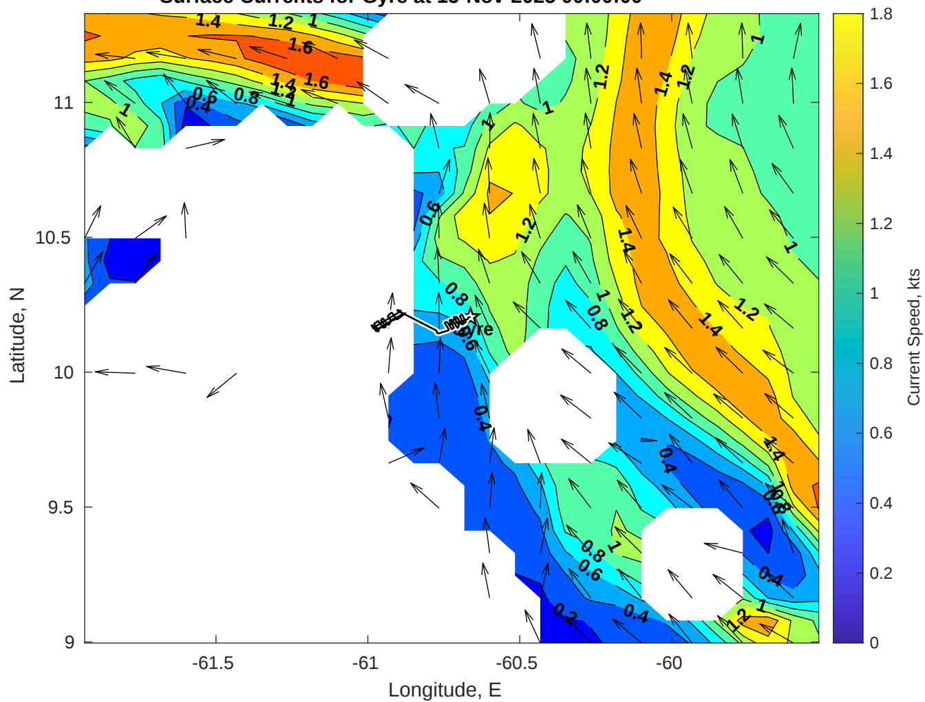
Surface Currents for Gyre at 15-Nov-2025 00:00:00
