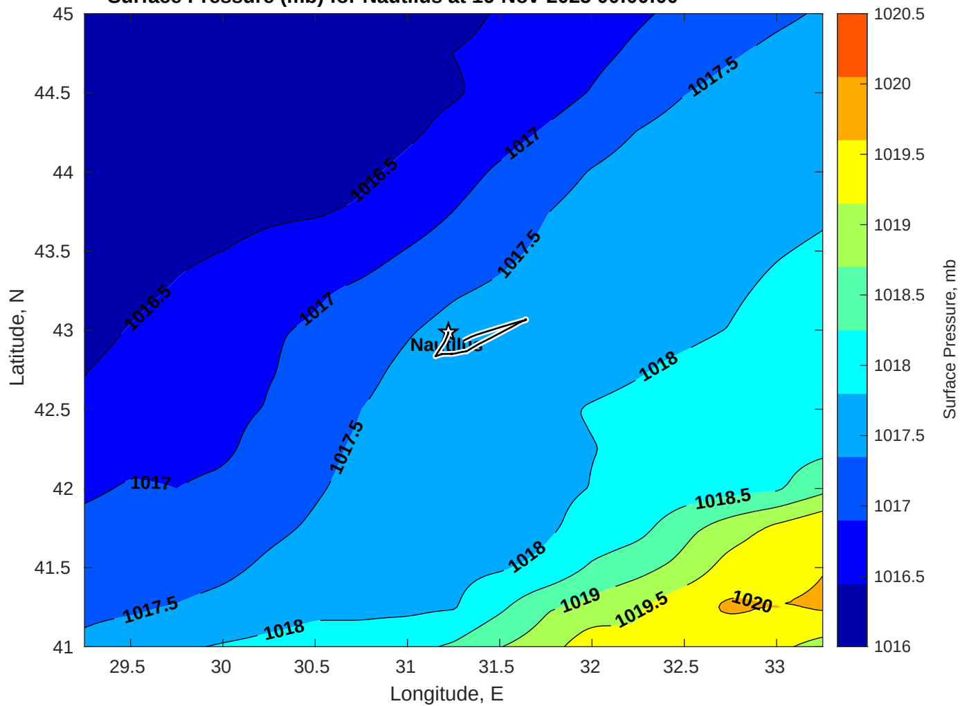
Surface Pressure (mb) for Nautilus at 16-Nov-2025 00:00:00
