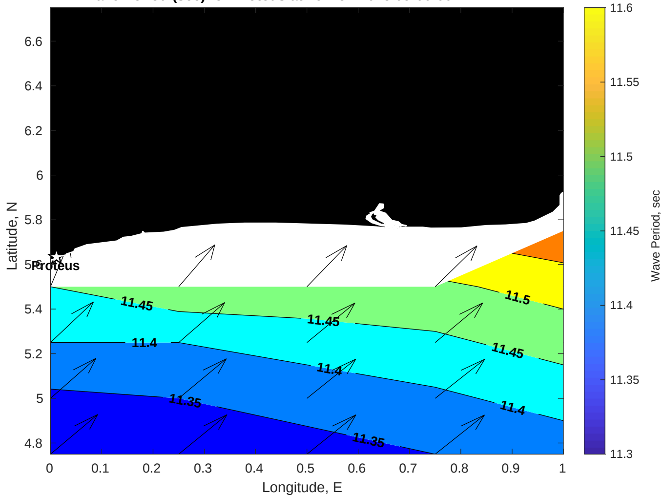
Wave Period (sec) for Proteus at 16-Nov-2025 09:00:00
