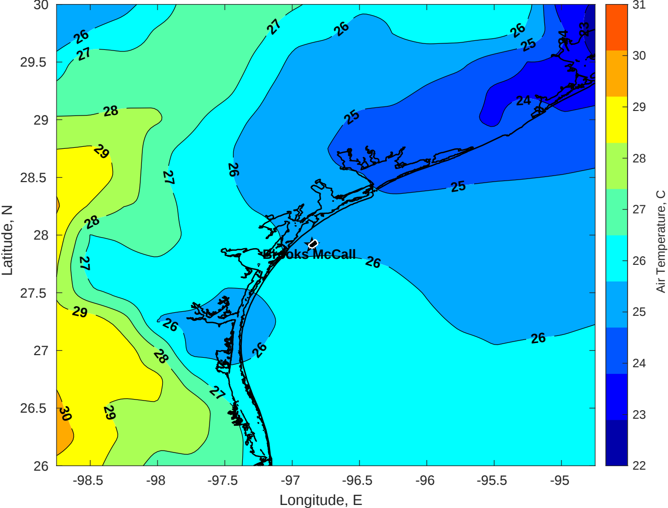
Air Temperature (C) for Brooks McCall at 17-Nov-2025
