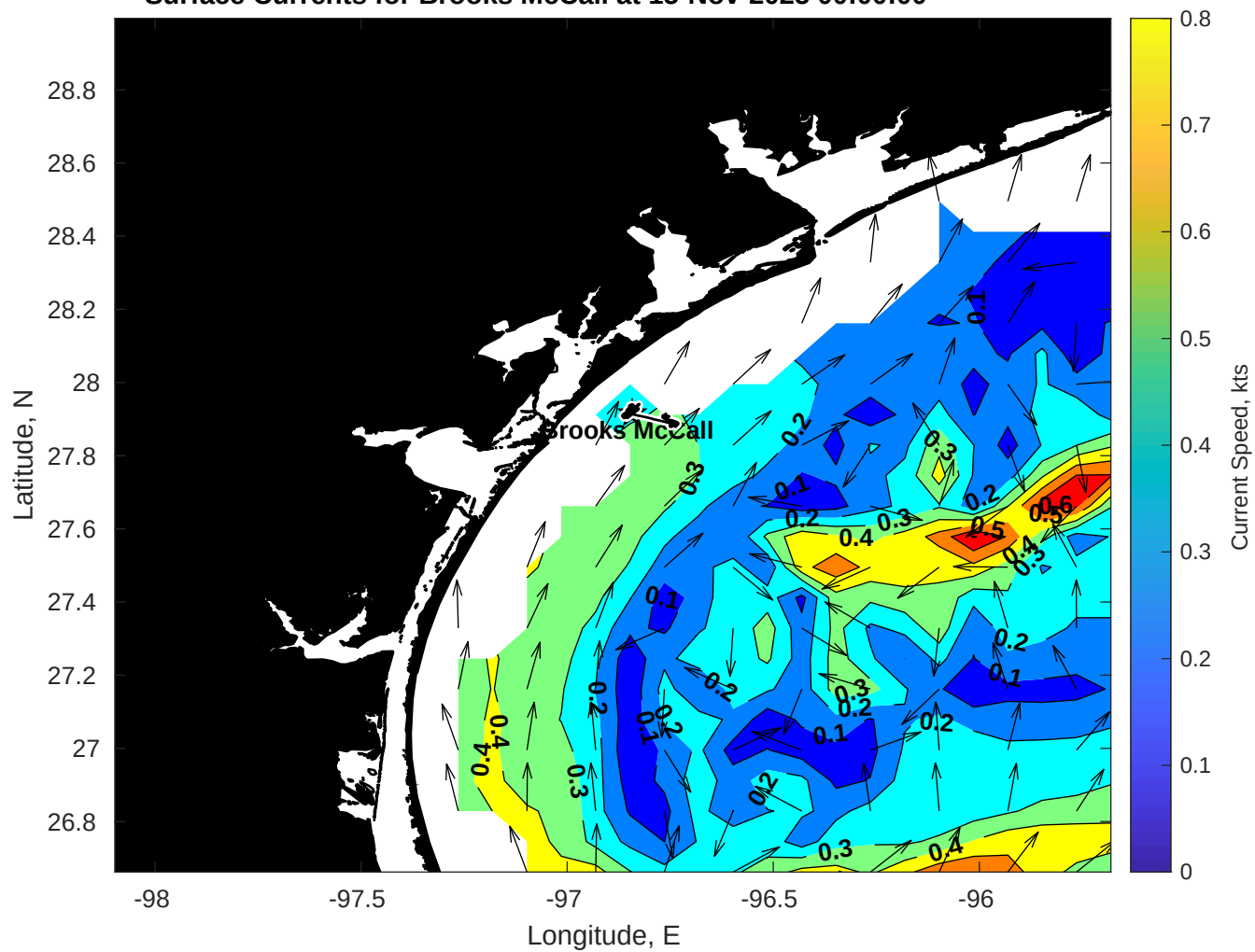
Surface Currents for Brooks McCall at 15-Nov-2025 00:00:00
